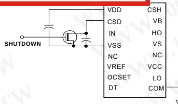
Figure 9: Shutdown Input
