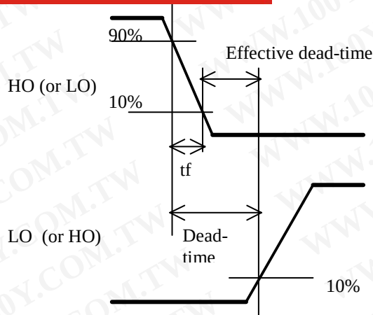
Figure 15: Effective Deadtime
