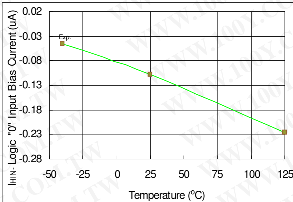
Figure 81. I HIN- Logic "0" Input Bias Current vs. Temperature
