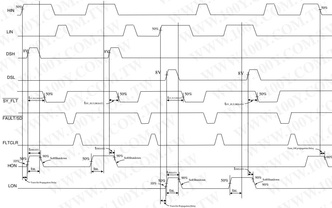
Figure 10: Desat Timing
