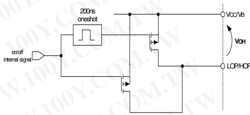
Figure 5: HOP and LOP Diagram
