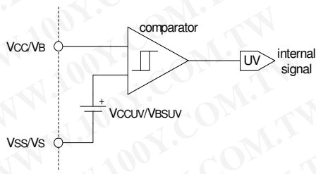
Figure 1: Undervoltage Diagram
