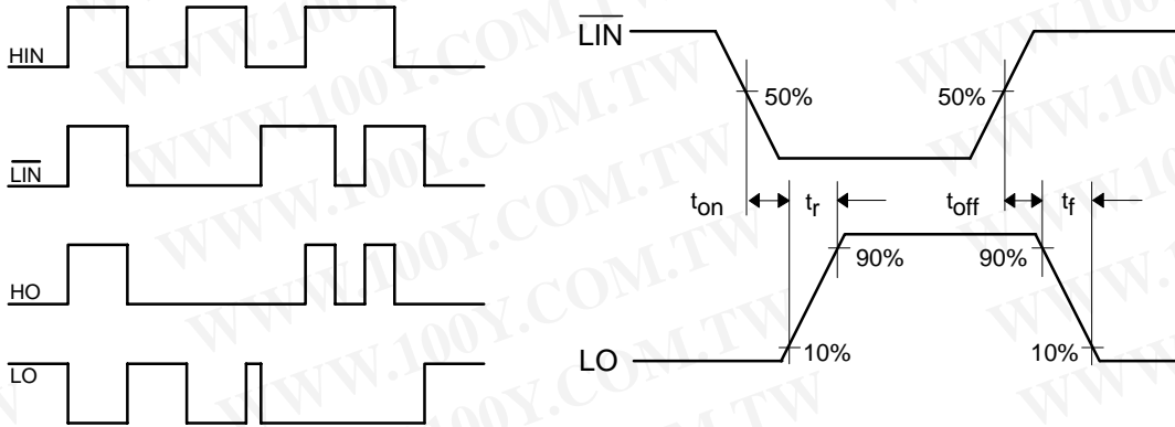
Figure 1. Input/Output Timing Diagram
