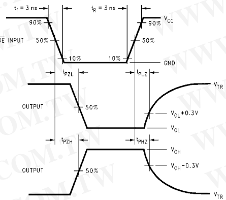
FIGURE 3. AC Waveforms
