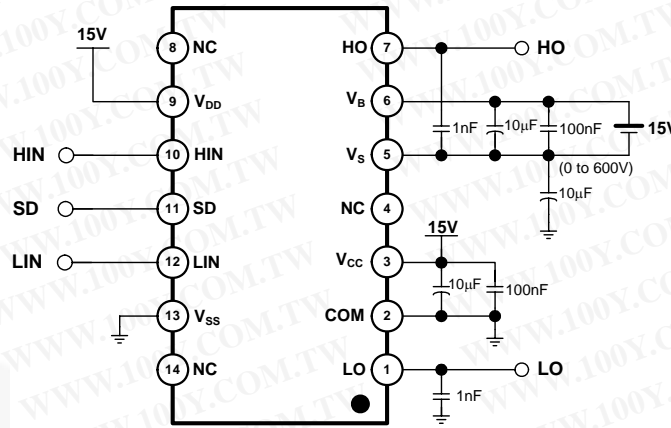
Figure 29. Switching Time Test Circuit (Referenced 14-DIP)
