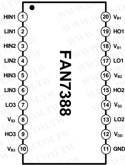
Figure 3. Pin Configuration (Top View)
