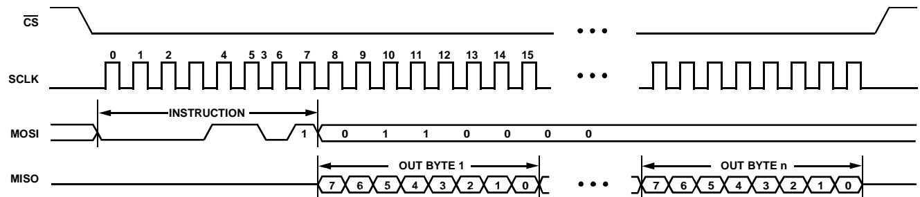
图40. FIFO读取
