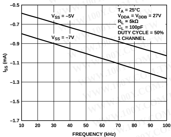
Figure 6. Supply Current ( I_{SS} ) vs. Frequency
