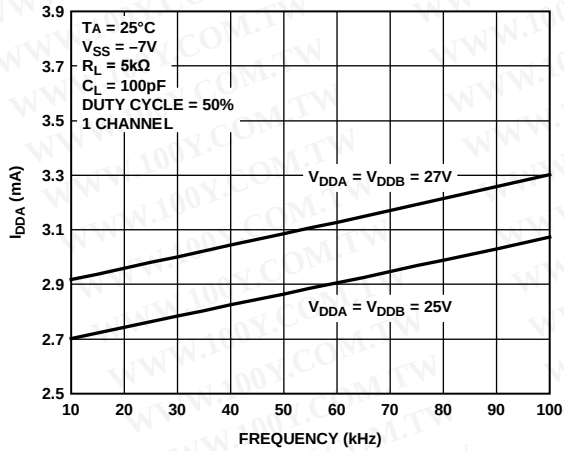
Figure 5. Supply Current ( I_{DDA} ) vs. Frequency
