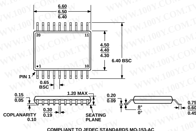
Figure 19. 20-Lead Thin Shrink Small Outline Package [TSSOP] (RU-20)
