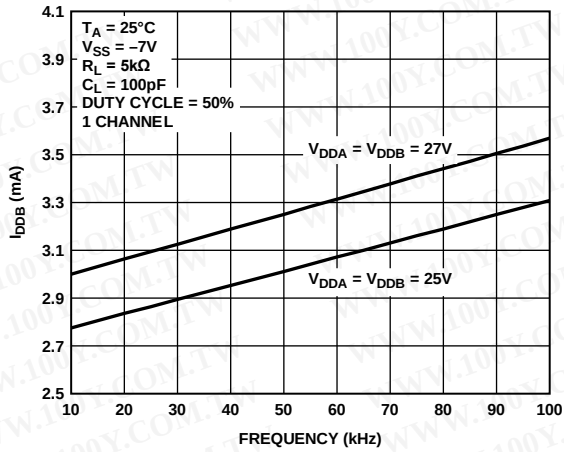
Figure 4. Supply Current ( I_{DDB} ) vs. Frequency
