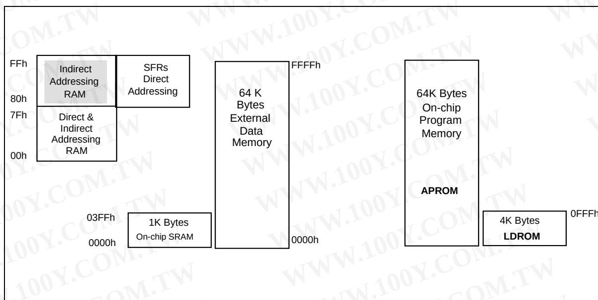
Figure 1. Memory Map
