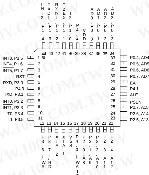
44-Pin QFP
