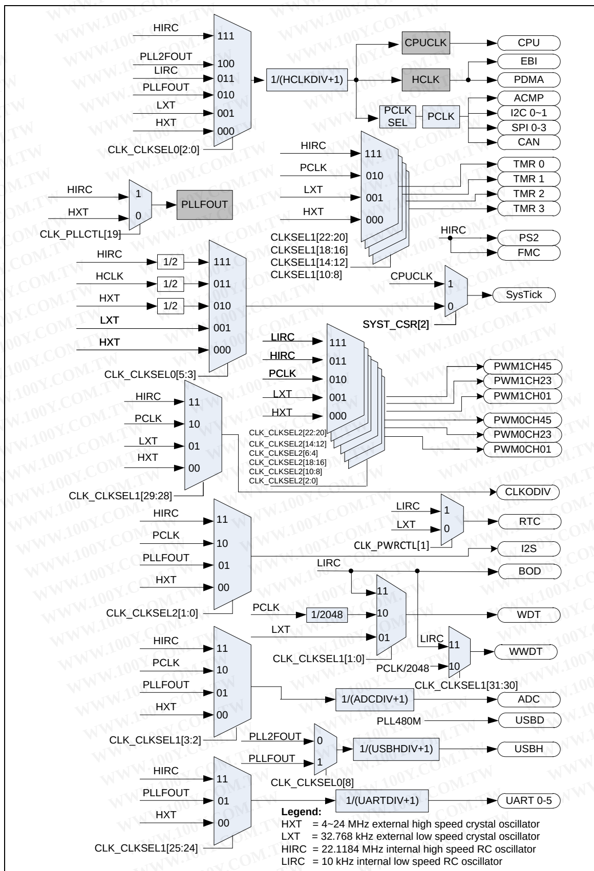
Figure 6.3-2 Clock Generator Global View Diagram
