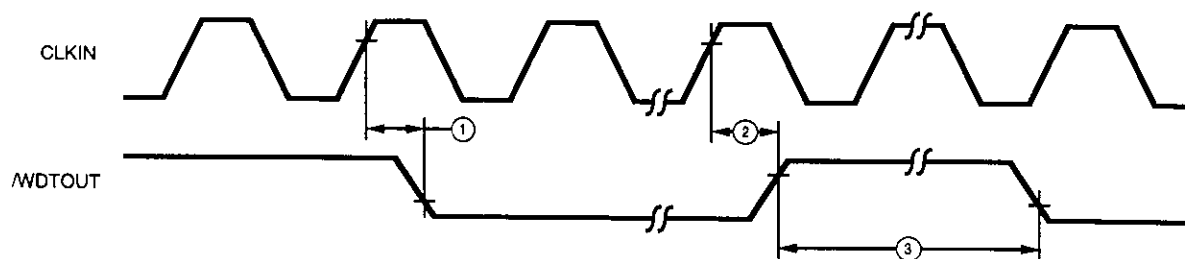
Watch-Dog Timer Timing (See Table H)
