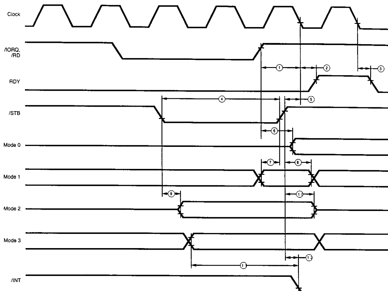
PIO Timing (See Table D)
