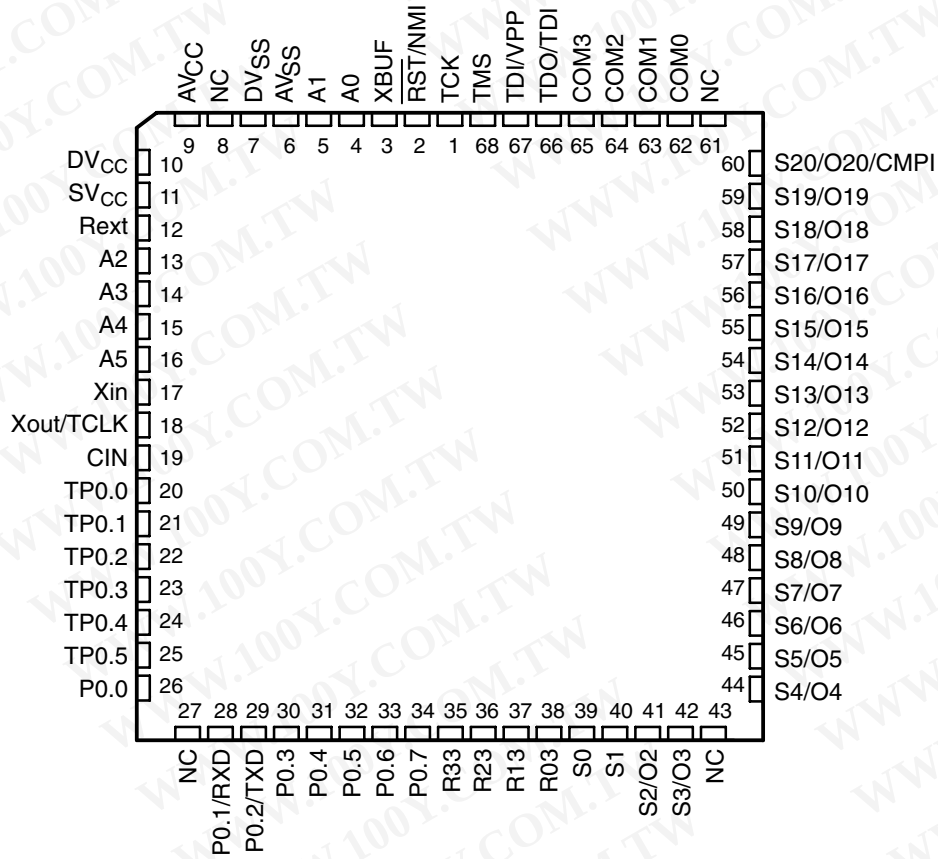
FN PACKAGE (TOP VIEW)
