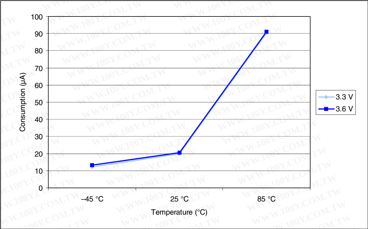
Figure 17. Typical current consumption in Stop mode with regulator in Low-power mode versus temperature at V_{DD} = 3.3\text{ V} and 3.6\text{ V}
