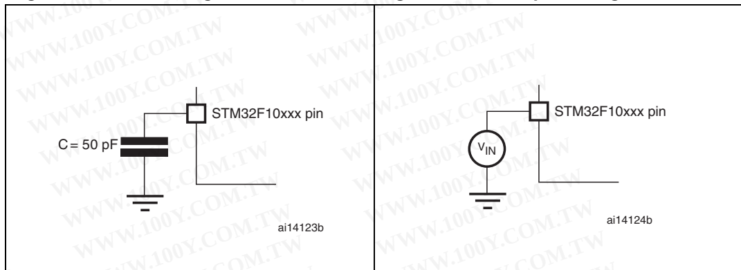
Figure 10. Pin input voltage
