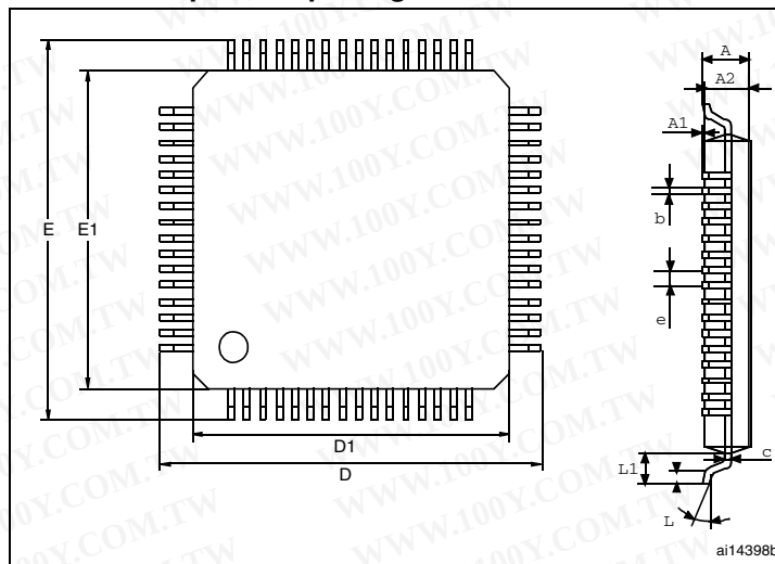
Figure 43. LQFP64 – 10 x 10 mm, 64 pin low-profile quad flat package outline (1)
