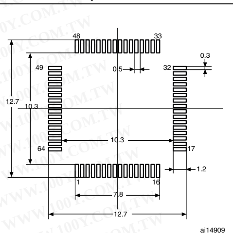
Figure 44. Recommended footprint (1)(2)
