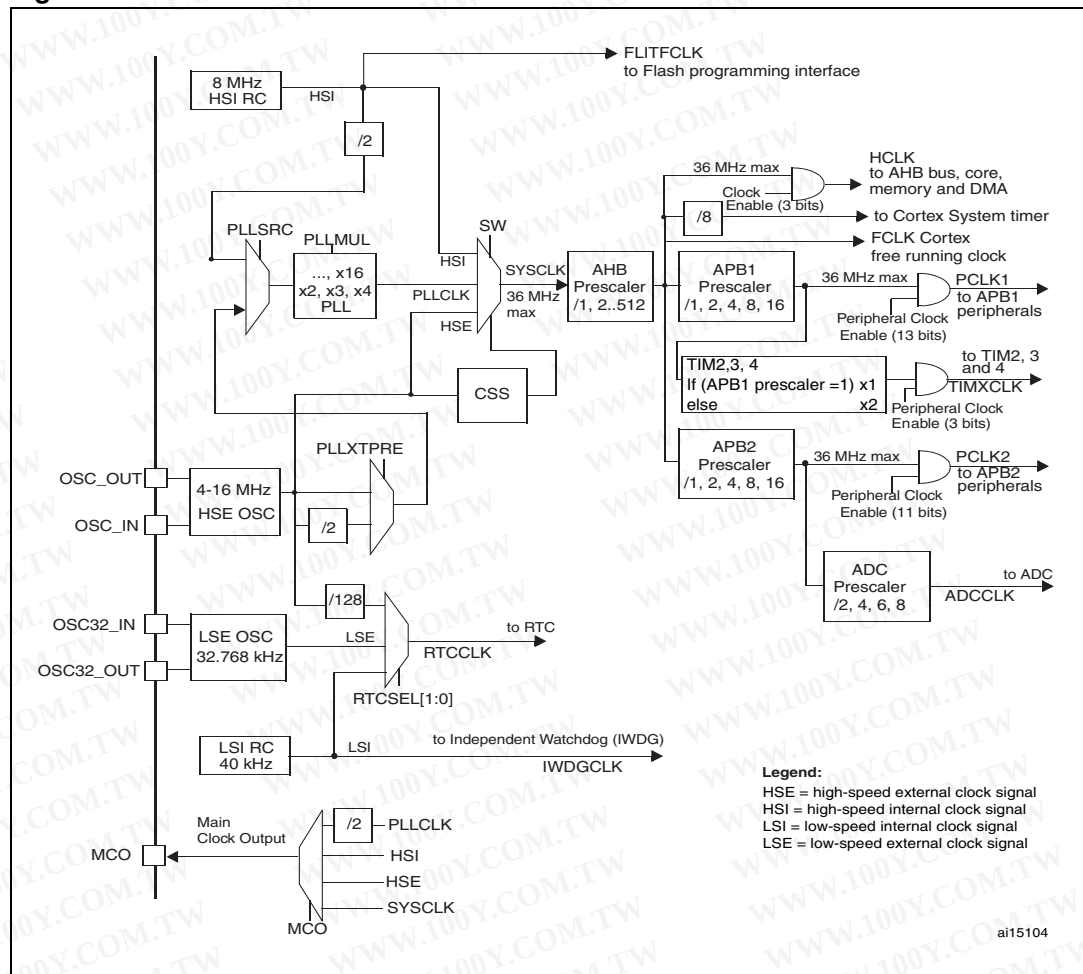
Figure 2. Clock tree
