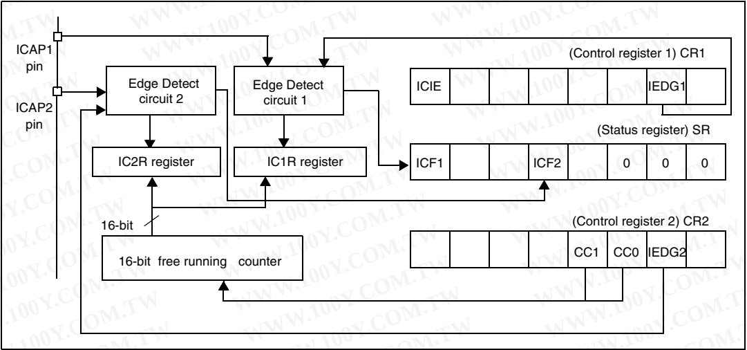
Figure 41. Input capture block diagram
