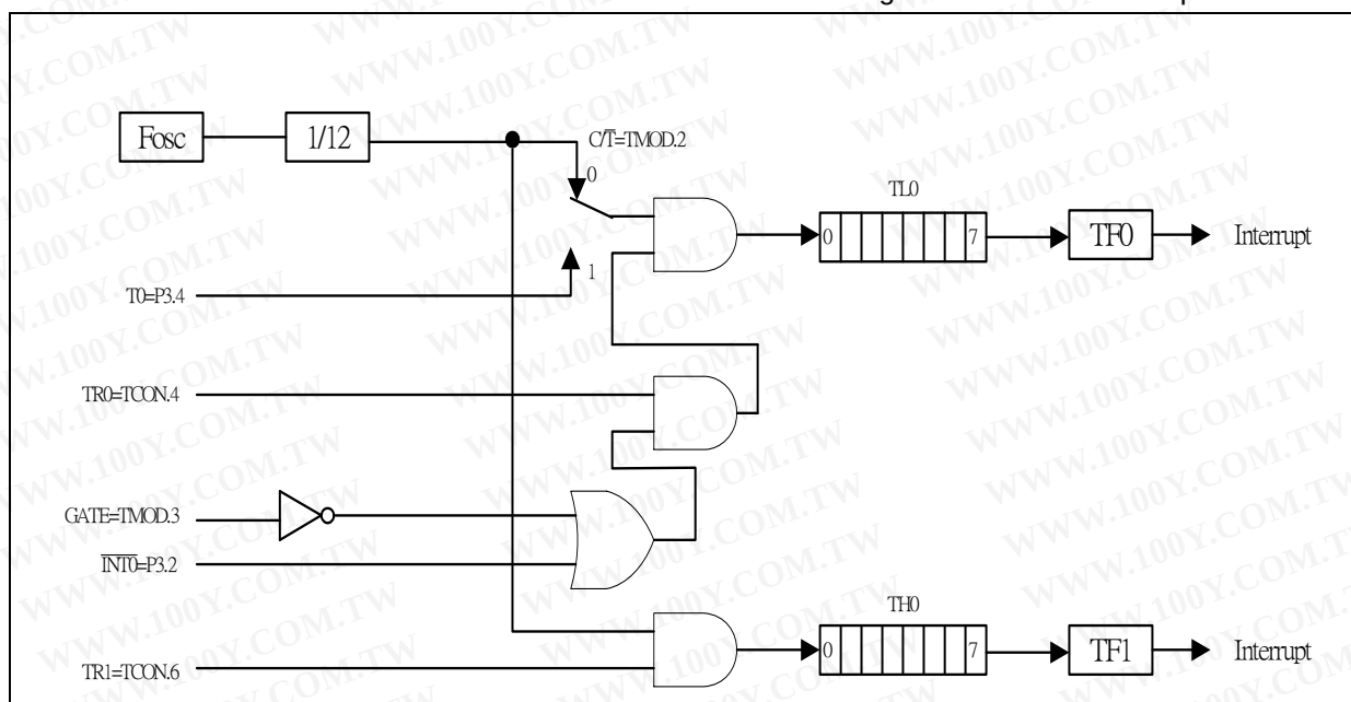
Figure 14- 3 Timer/Counter Mode 3
