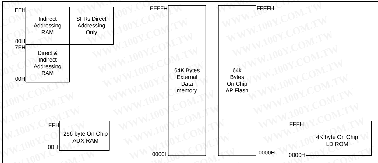
Figure 8- 1 Memory Map
