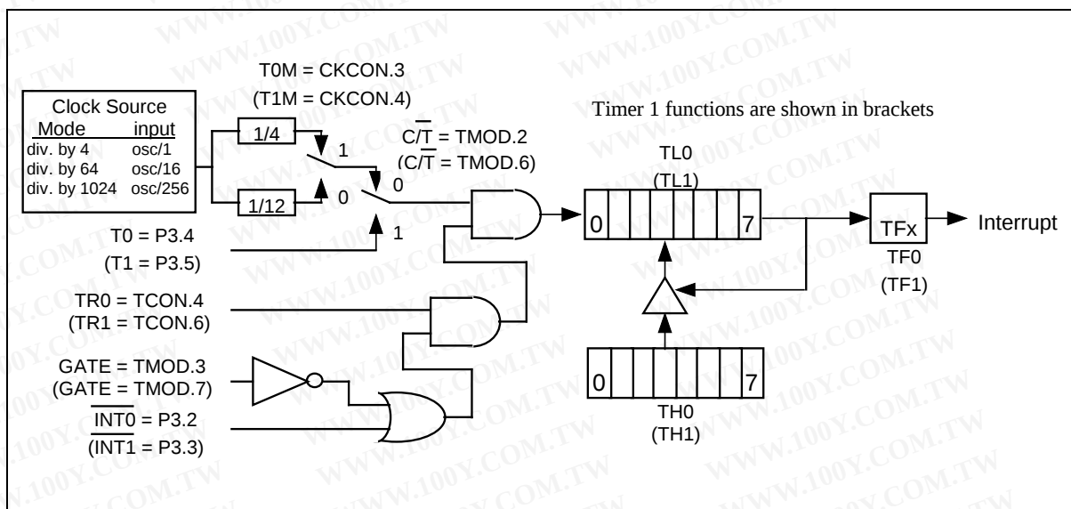
Figure 12. Timer/Counter Mode 2.
