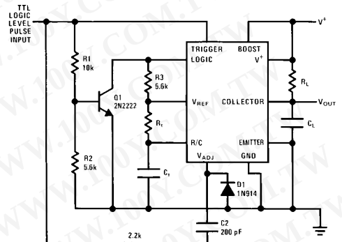
* V_{OUT} = 0 for W \cdot R_1 \cdot C_1 Pulse Out = W - R_1 \cdot C_1 for W \cdot R_1 \cdot C_1 FIGURE 12. Pulse Width Detector
