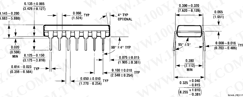
Dual-In-Line Package (N) Order Number LM322N NS Package Number N14A
