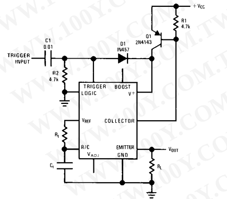
FIGURE 10. Zero Power Dissipation Between Timing Intervals
