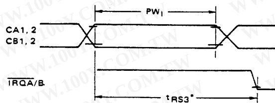
FIGURE 13 — INTERRUPT PULSE WIDTH AND \overline{IRQ} RESPONSE
