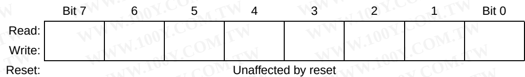
Figure 4-2. Accumulator (A)
