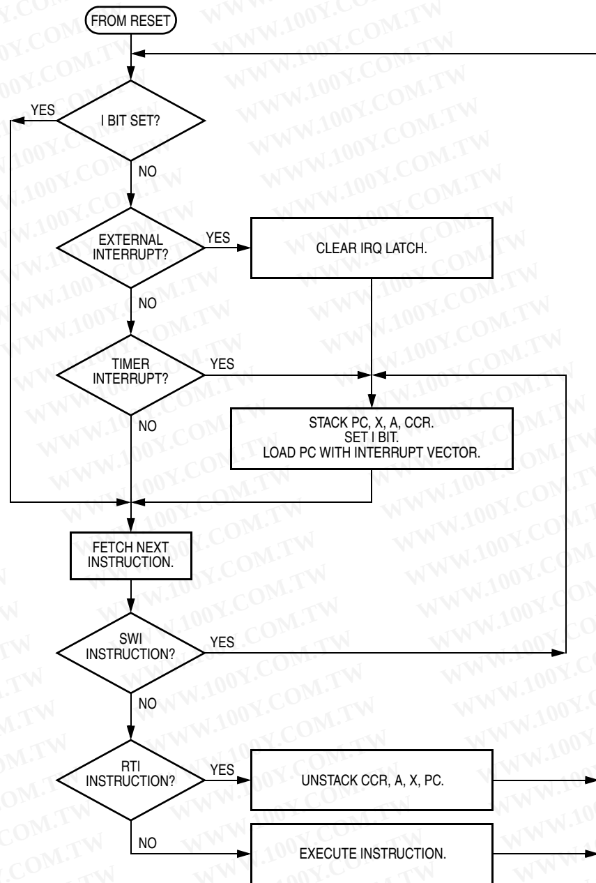
Figure 8-7. Interrupt Flowchart
