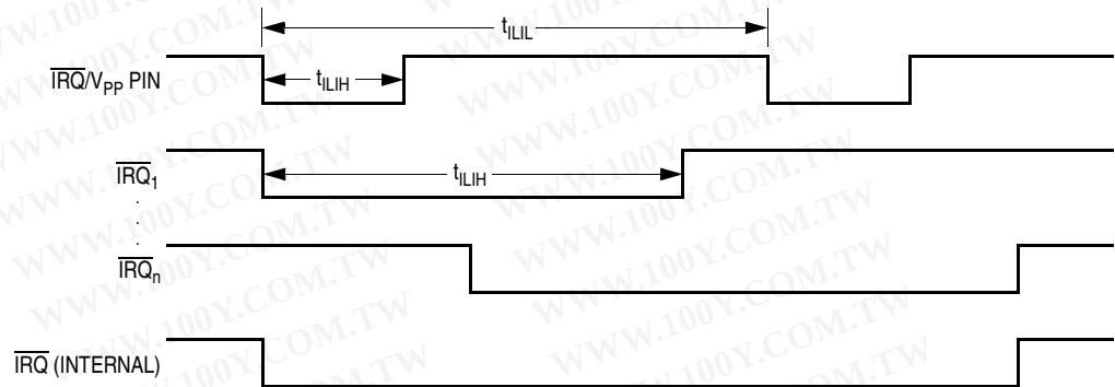
Figure 5-5. External Interrupt Timing
