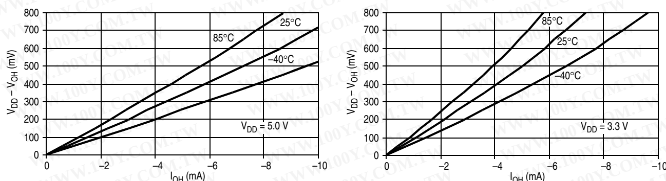
Figure 10-1. PA4-PA7 Typical High-Side Driver Characteristics
