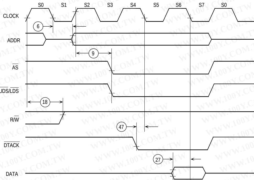
Figure 5-35. Synchronous Read Cycle
