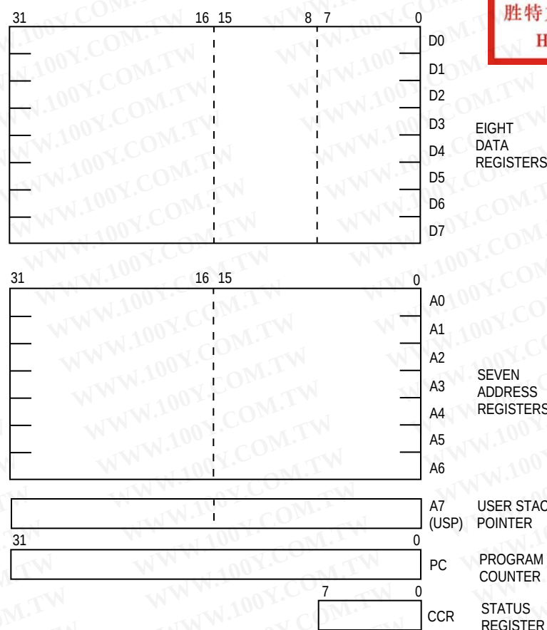
Figure 2-1. User Programmer's Model (MC68000/MC68HC000/MC68008/MC68010)
