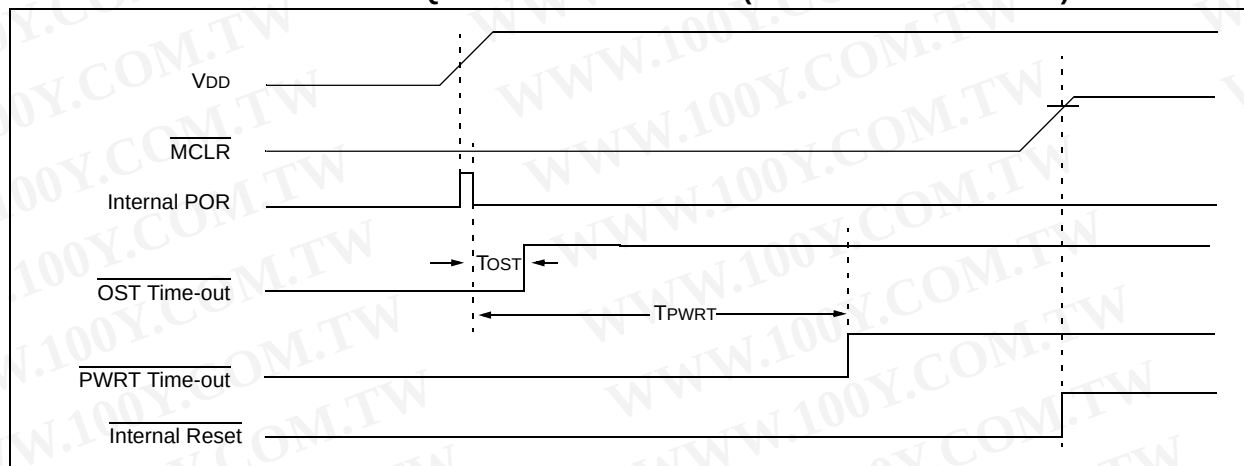
FIGURE 21-5: TIME-OUT SEQUENCE ON POWER-UP (MCLR NOT TIED TO VDD): CASE 2
