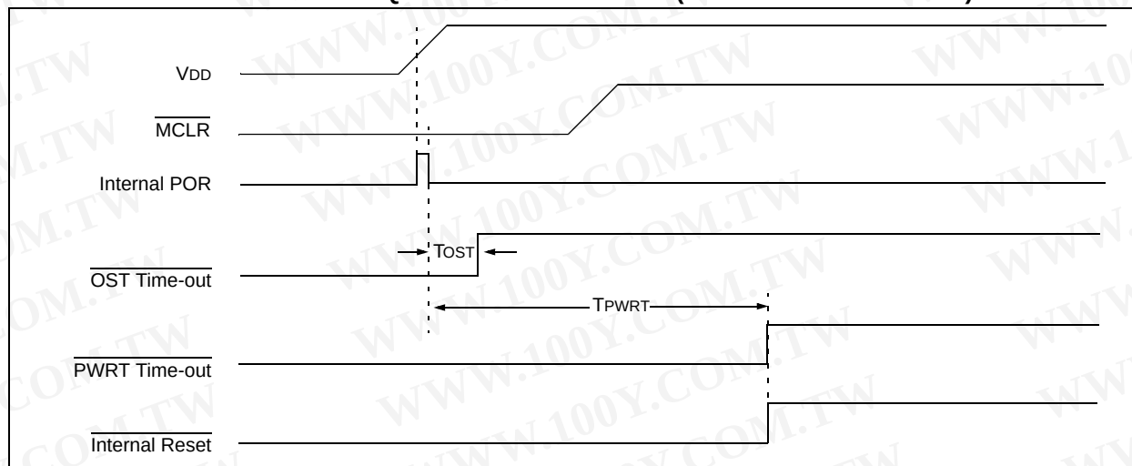
FIGURE 21-4: TIME-OUT SEQUENCE ON POWER-UP (MCLR NOT TIED TO VDD): CASE 1
