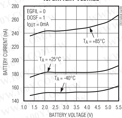
DS1343 BATTERY CURRENT1 vs. BATTERY VOLTAGE
