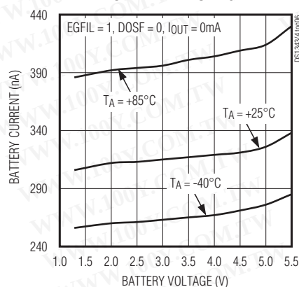
DS1344 BATTERY CURRENT2 vs. BATTERY VOLTAGE
