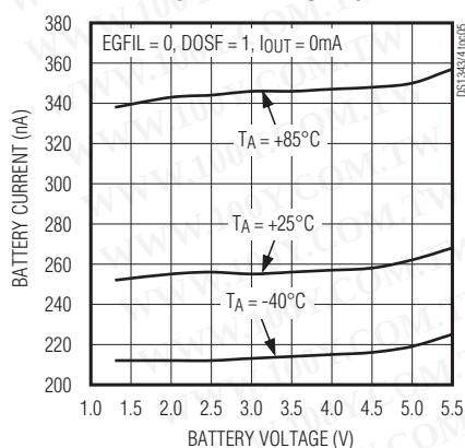
DS1344 BATTERY CURRENT1 vs. BATTERY VOLTAGE
