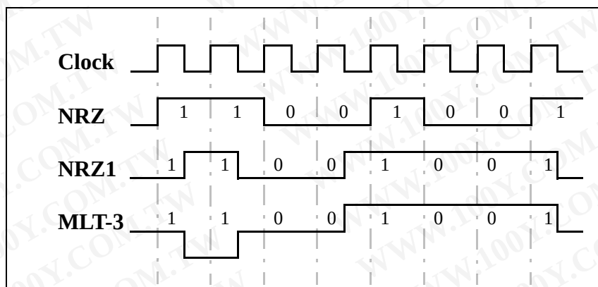
Figure 13. NRZ to MLT-3 Encoding Diagram
