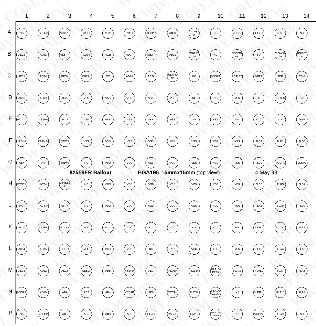
Figure 34. 82559ER Ball Grid Array Diagram
