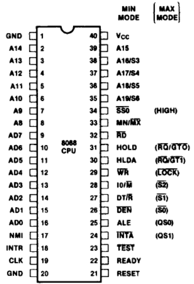
Figure 2. 8088 Pin Configuration
