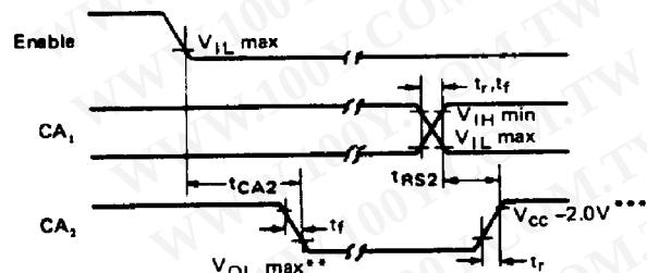
Figure 3 CA 2 Delay Time (Read Mode; CRA5=1, CRA3=CRA4=0)
