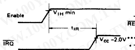
Figure 9 \overline{\text{IRQ}} Release Time
