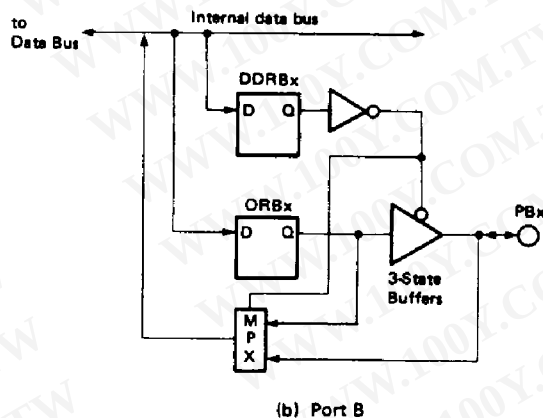
Figure 15 Block Diagram of Port A and Port B (HD6321)
