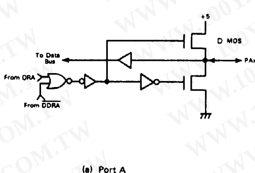
Figure 16 Circuit of Port A and Port B (HD6821)
