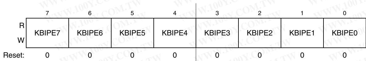
Figure 10-4. KBI Pin Enable Register
