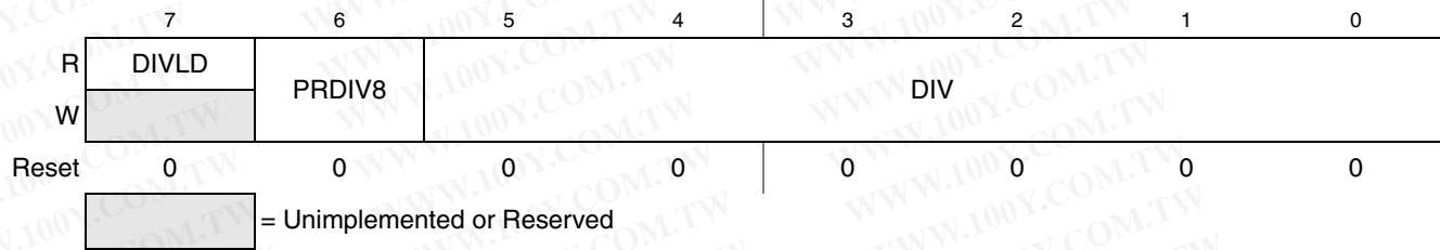
Figure 4-5. Flash Clock Divider Register (FCDIV)
