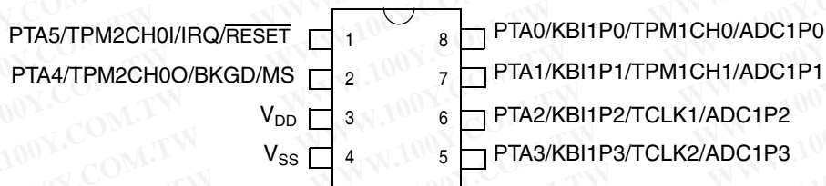
Figure 2-1. 8-Pin Packages
