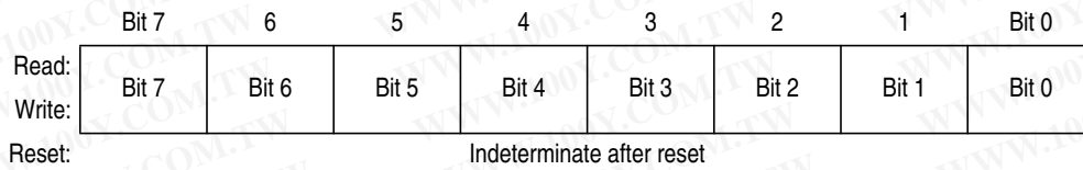
Figure 16-15. TIM1 Channel Register Low (T1CHxL)
