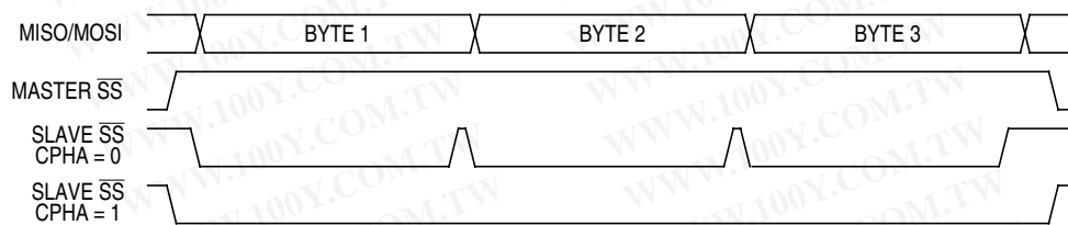
Figure 15-5. CPHA/\overline{SS} Timing
