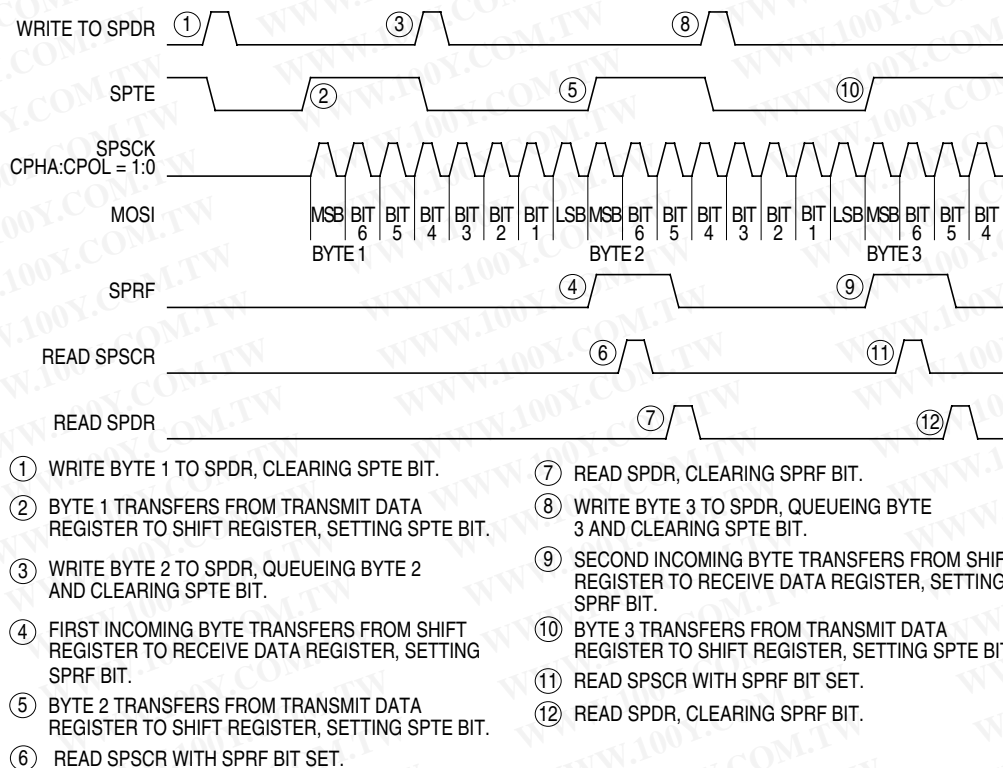
Figure 15-8. SPRF/SPTE interrupt Timing
