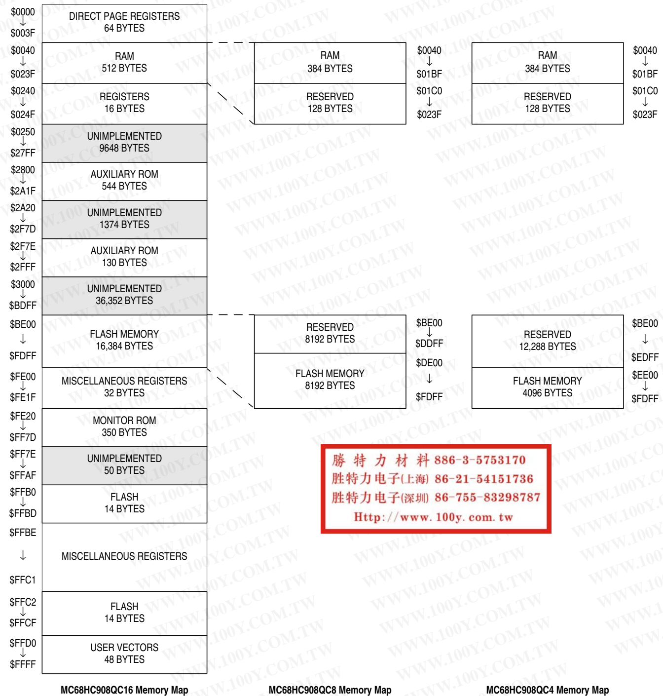
Figure 2-1. Memory Map
