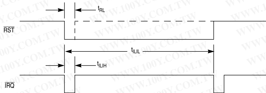
Figure 19-3. RST and IRQ Timing
