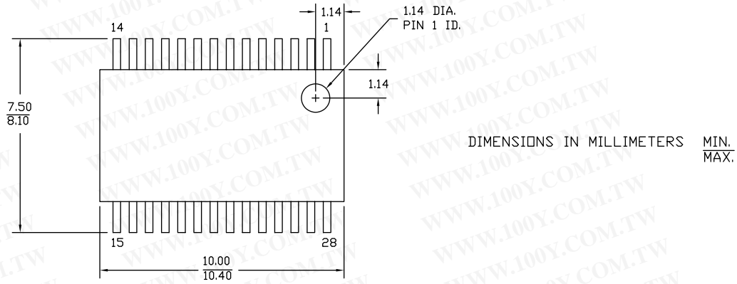
Figure 11. 28-Pin SSOP Package Outline
