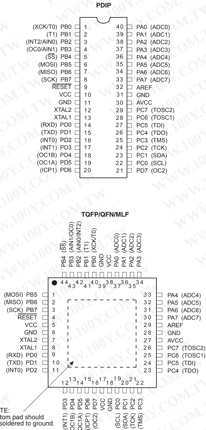
Figure 1-1. Pinout ATmega16A
