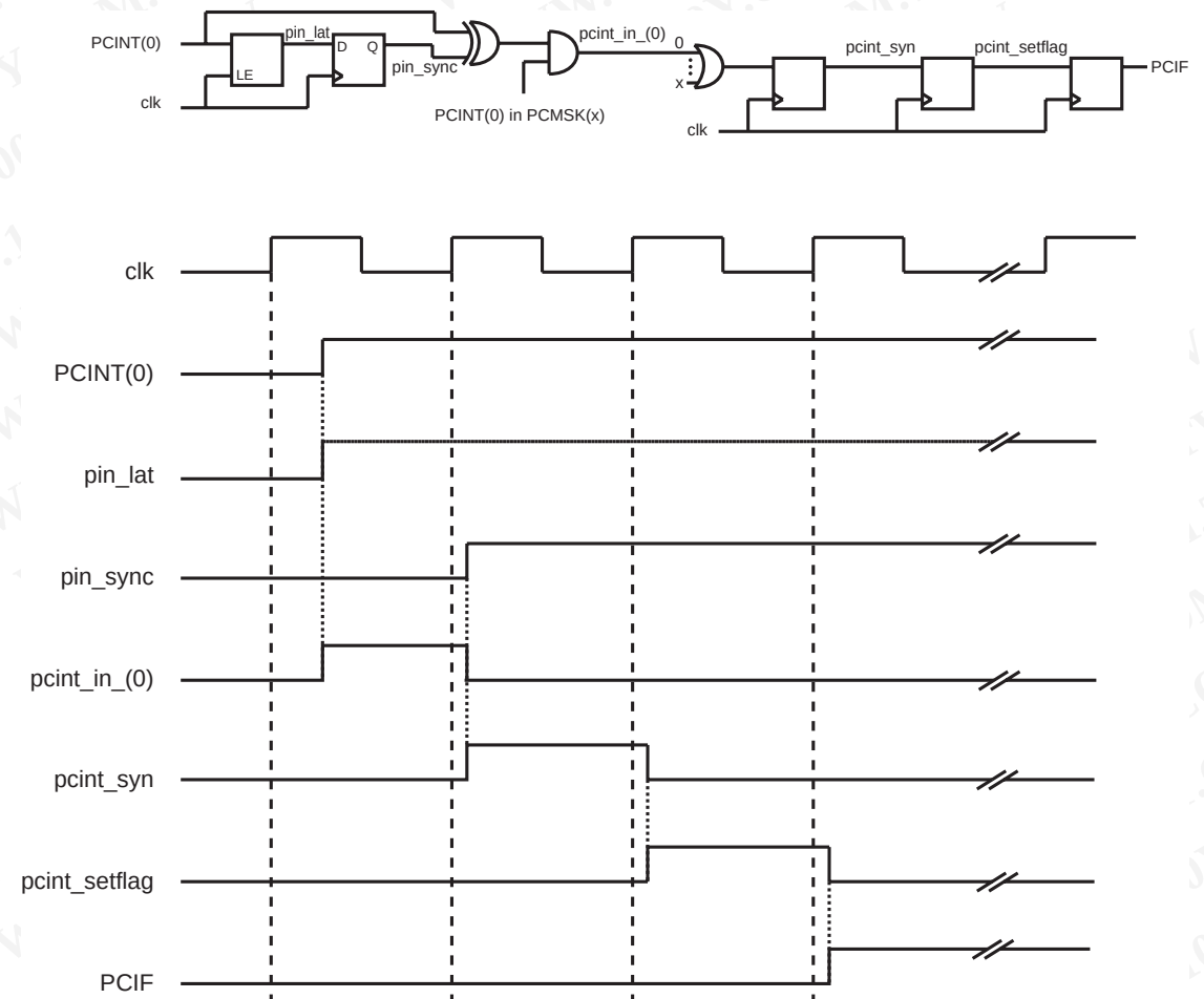
Figure 9-1. Timing of pin change interrupts
