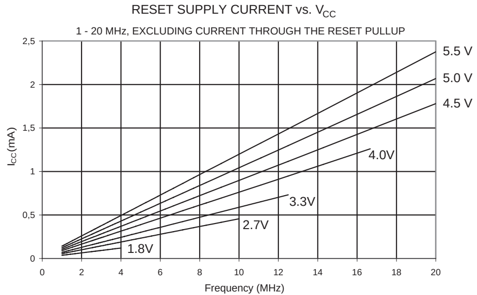
Figure 22-49. Reset Supply Current vs. V_{CC} (1 - 20 MHz, Excluding Current Through The Reset Pull-up)
