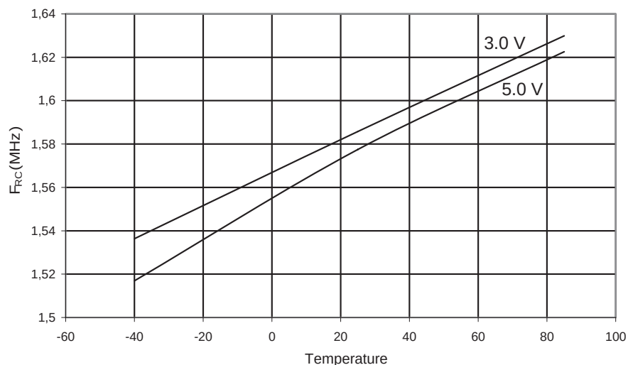
Figure 22-43. Calibrated 1.6 MHz RC Oscillator Frequency vs. OSCCAL Value
