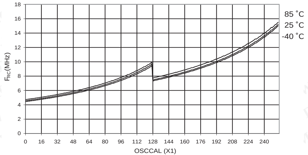
Figure 22-41. Calibrated 1.6 MHz RC Oscillator Frequency vs. V_{CC}
