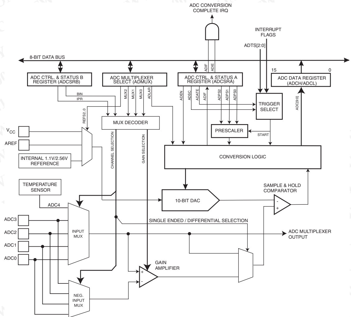
Figure 17-1. Analog to Digital Converter Block Schematic
