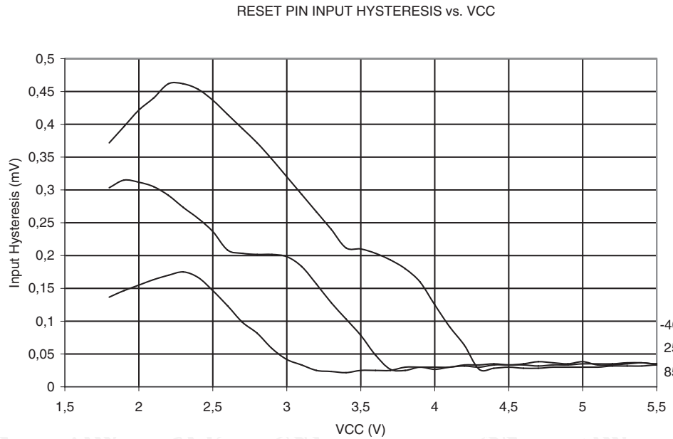
Figure 22-32. Reset Pin Input Hysteresis vs. V_{CC}
