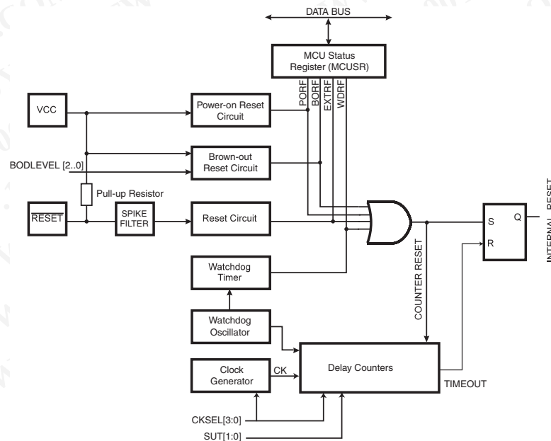
Figure 8-1. Reset Logic
