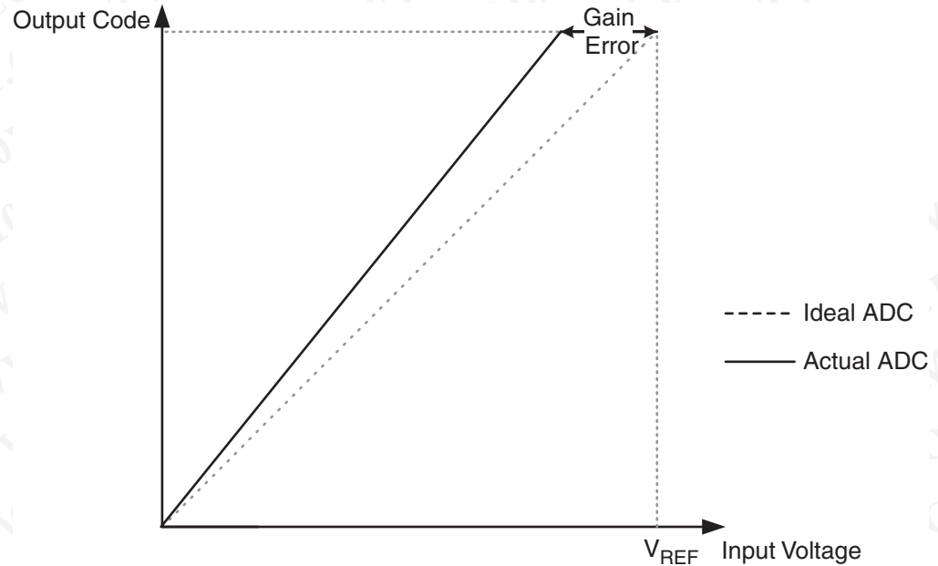
Figure 17-10. Gain Error
