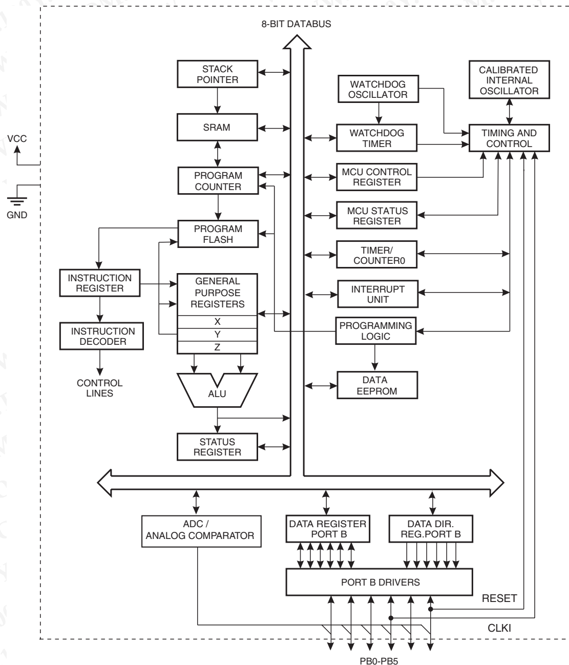
Figure 2-1. Block Diagram
