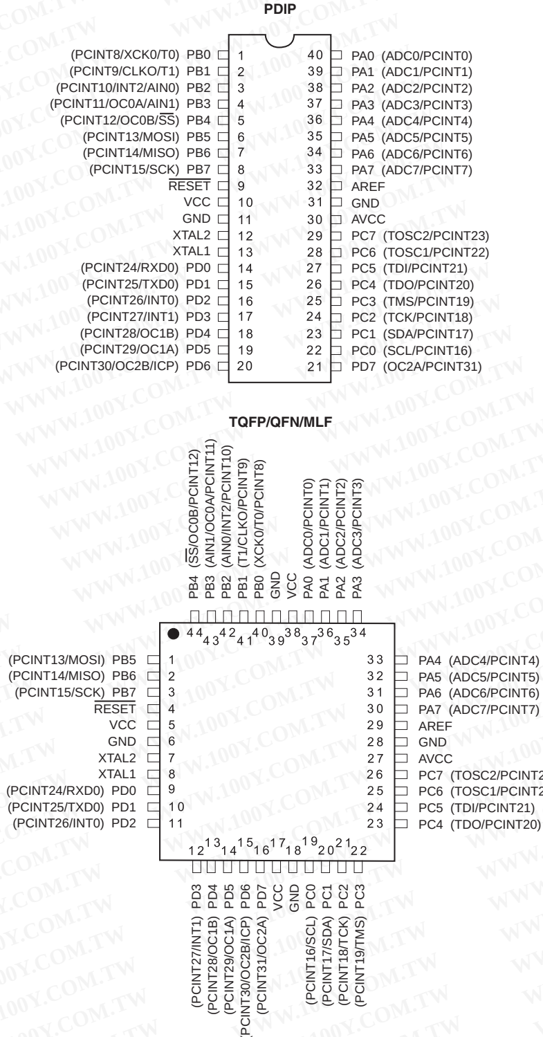
Figure 1-1. Pinout ATmega644
