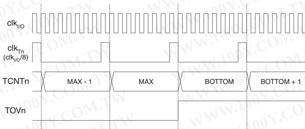
Figure 17-9. Timer/Counter Timing Diagram, with Prescaler ( f_{clk\_I/O}/8 )
