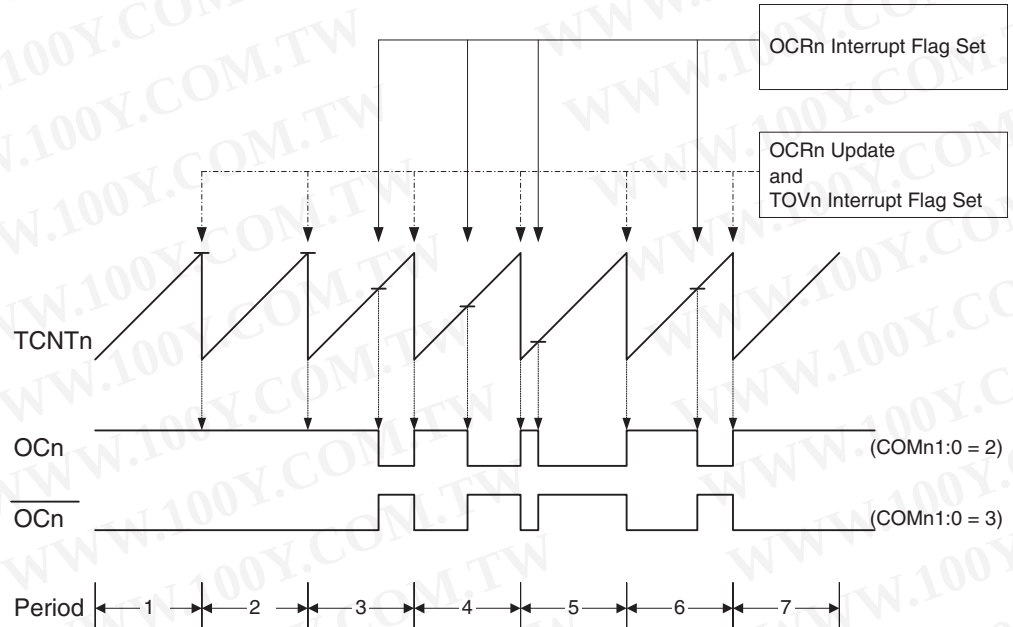
Figure 14-6. Fast PWM Mode, Timing Diagram
