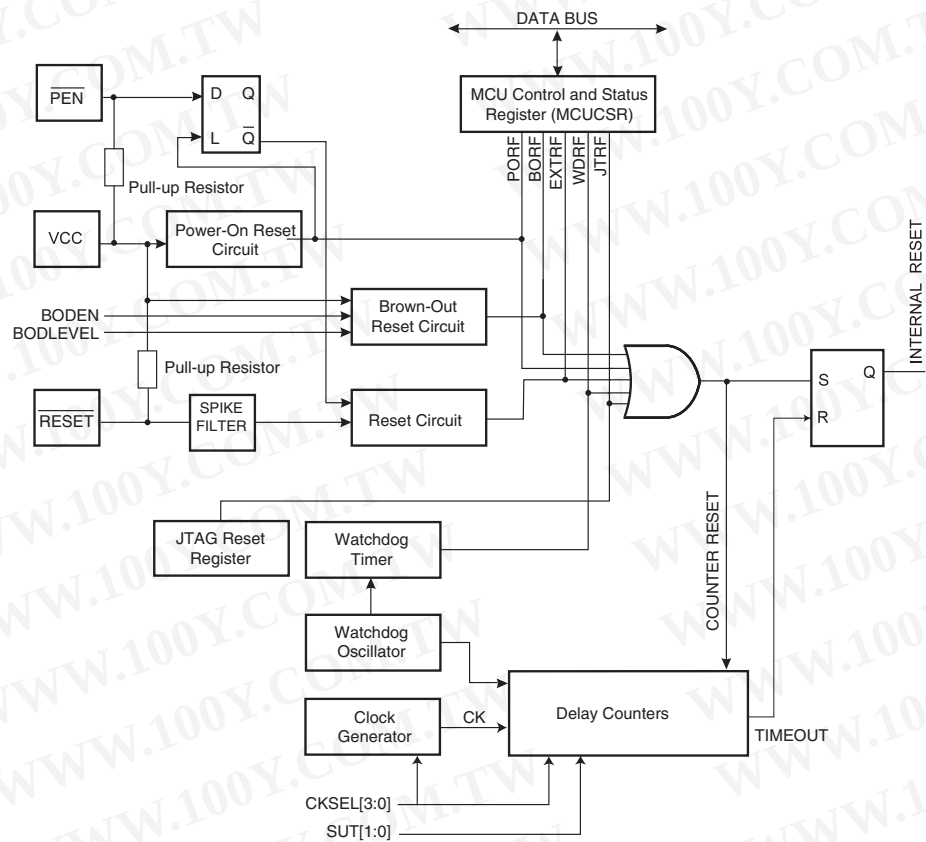
Figure 10-1. Reset Logic
