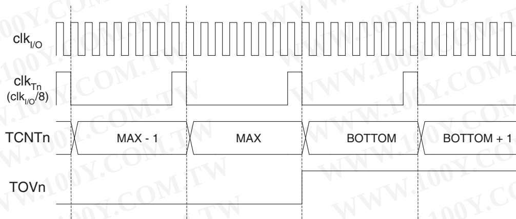
Figure 14-9. Timer/Counter Timing Diagram, with Prescaler ( f_{clk\_I/O}/8 )
