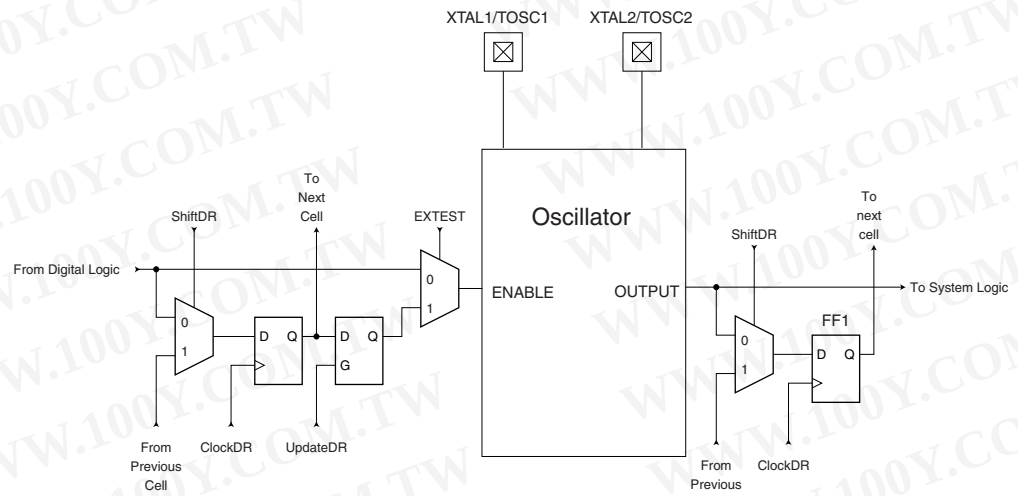
Figure 24-9. Boundary-scan Cells for Oscillators and Clock Options
