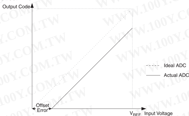
Figure 23-8. Offset Error
