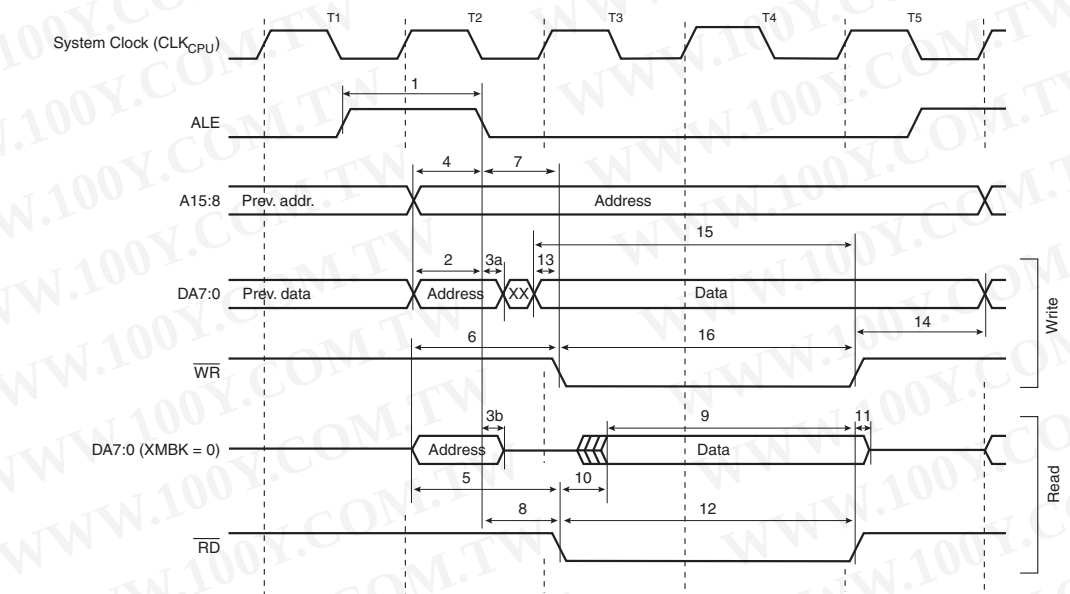
Figure 27-10. External Memory Timing (SRWn1 = 0, SRWn0 = 1)
