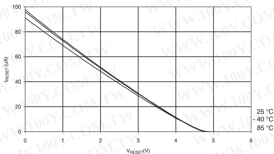
Figure 28-52. Reset Pull-up Resistor Current vs. Reset Pin Voltage ( V_{CC} = 5.0V )
