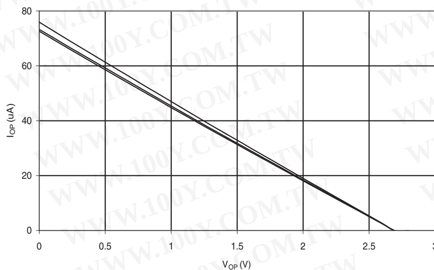
Figure 28-21. I/O Pin Pull-up Resistor Current vs. Input Voltage ( V_{CC} = 2.7V )
