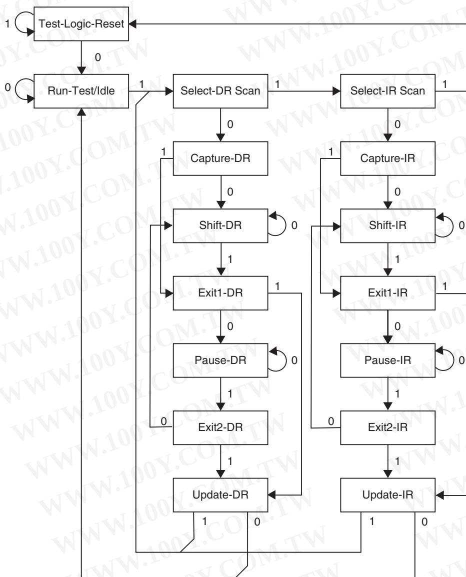
Figure 24-2. TAP Controller State Diagram
