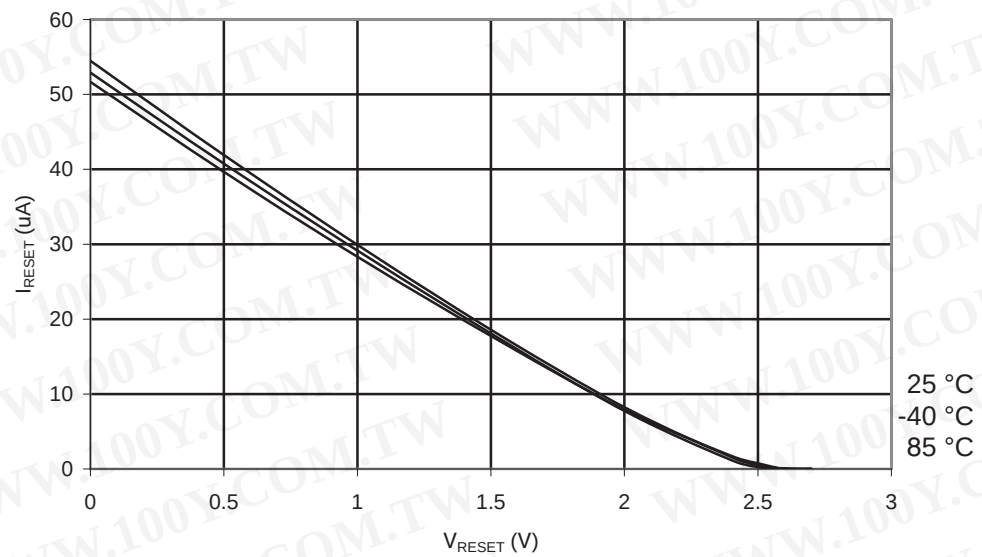
Figure 27-19. ATmega1284P: Reset Pull-up Resistor Current vs. Reset Pin Voltage ( V_{CC} = 2.7V ).
