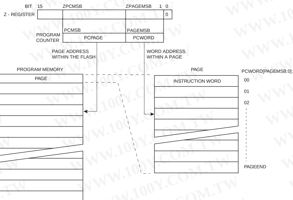
Figure 24-3. Addressing the Flash During SPM (1)
