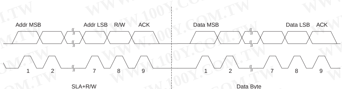
Figure 19-6. Typical Data Transmission
