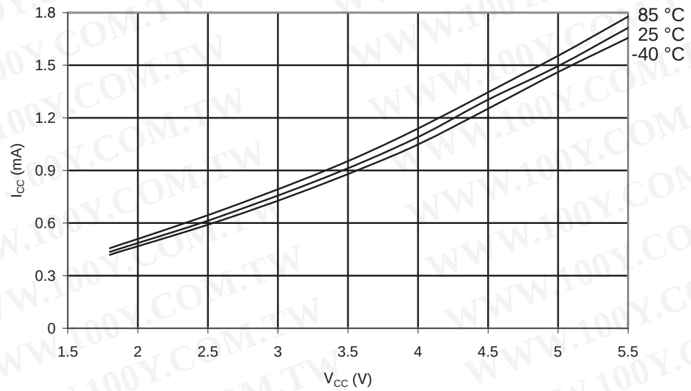
Figure 27-5. ATmega1284P: Active Supply Current vs. V_{CC} (Internal RC Oscillator, 128 kHz)
