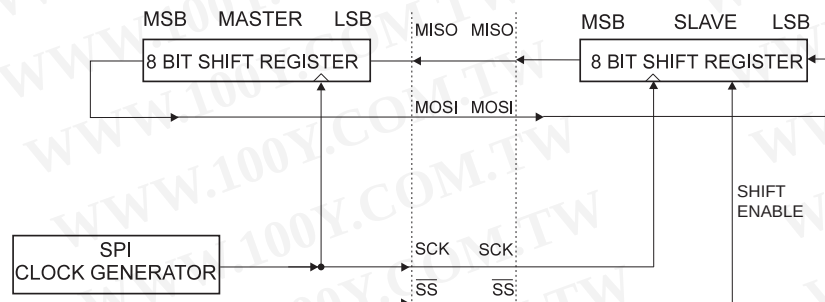
Figure 16-2. SPI Master-slave Interconnection
