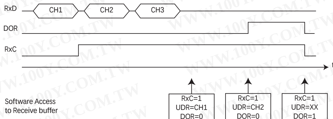
Figure 18-5. Data OverRun example
