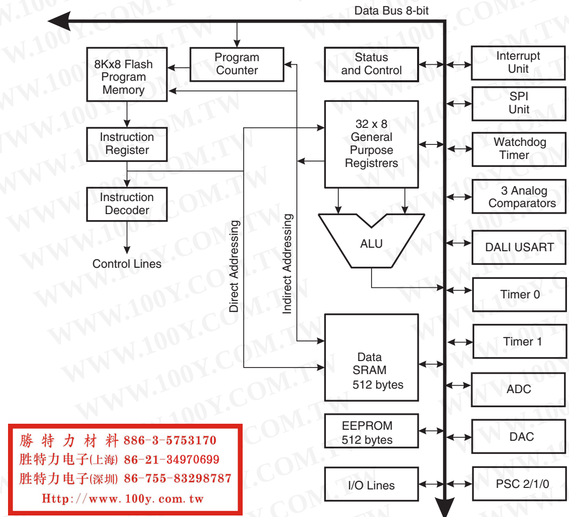
Figure 4-1. Block Diagram
