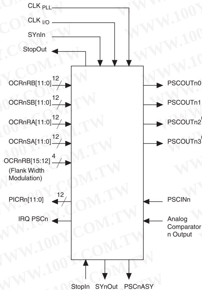
Figure 16-3. PSC External Block View
