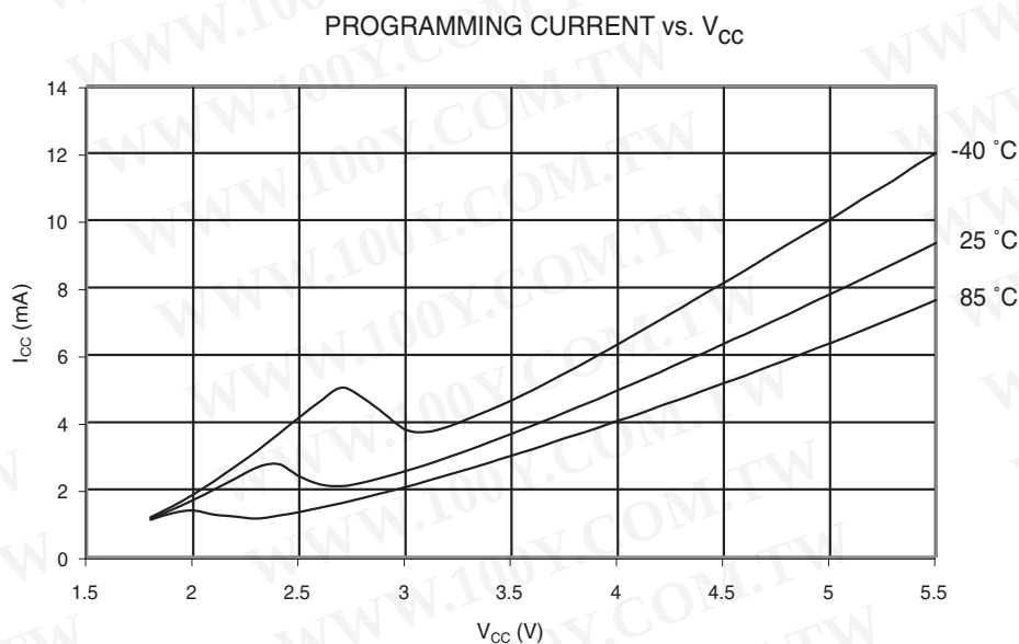
Figure 27-43. Programming Current vs. V_{CC}
