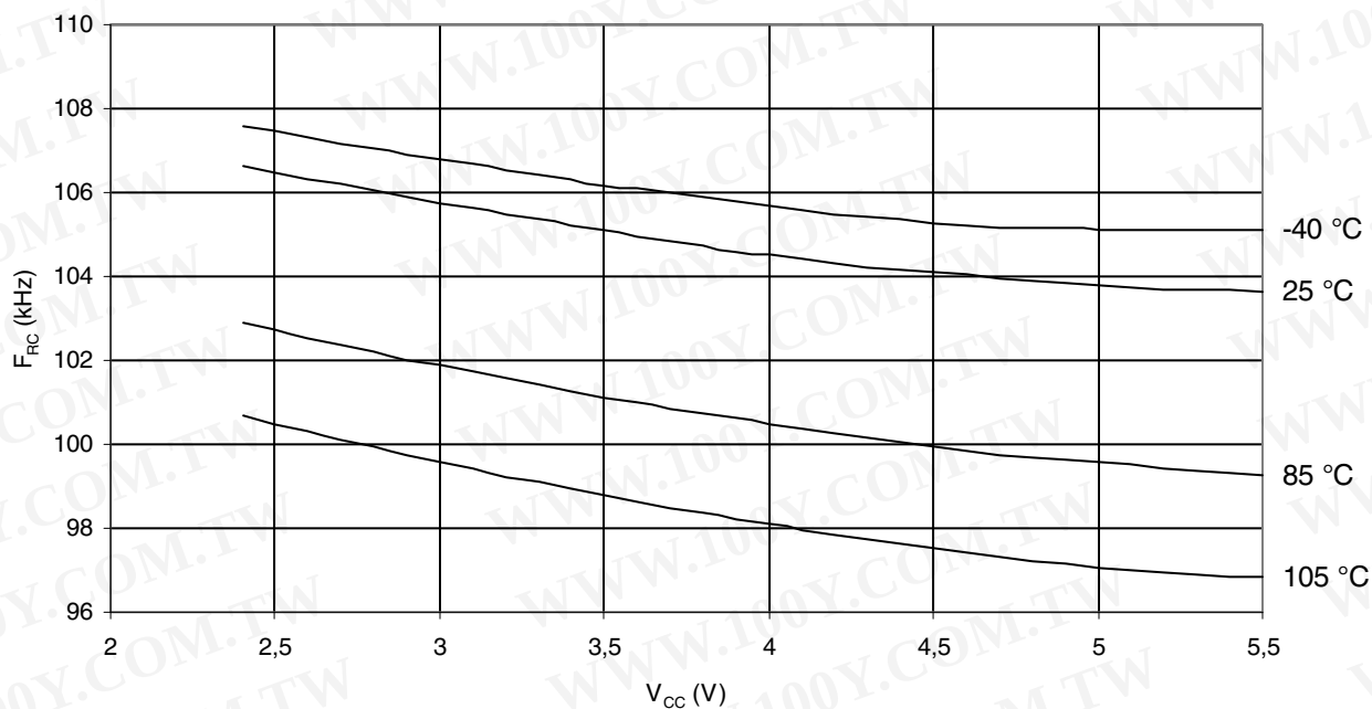
Figure 27-35. Watchdog Oscillator Frequency vs. V CC
