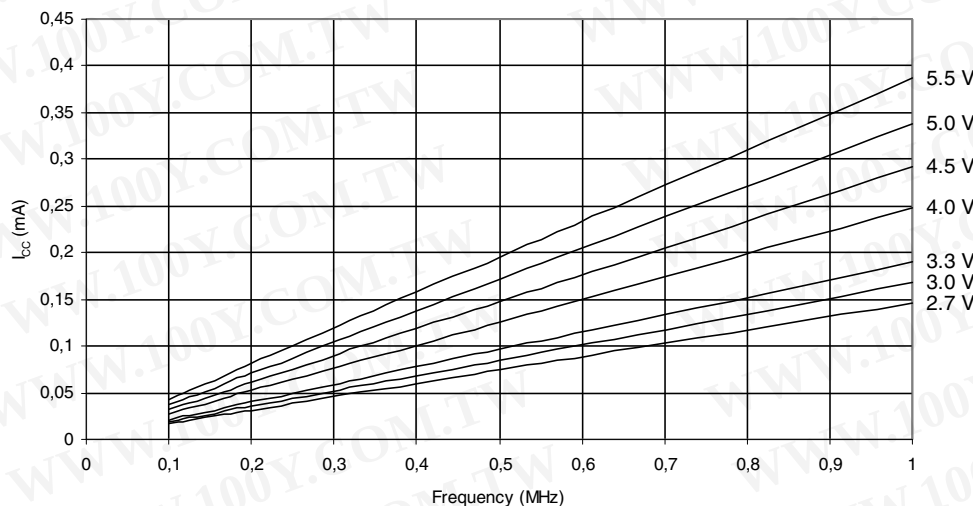
Figure 27-6. Idle Supply Current vs. Frequency (1 - 24 MHz)
