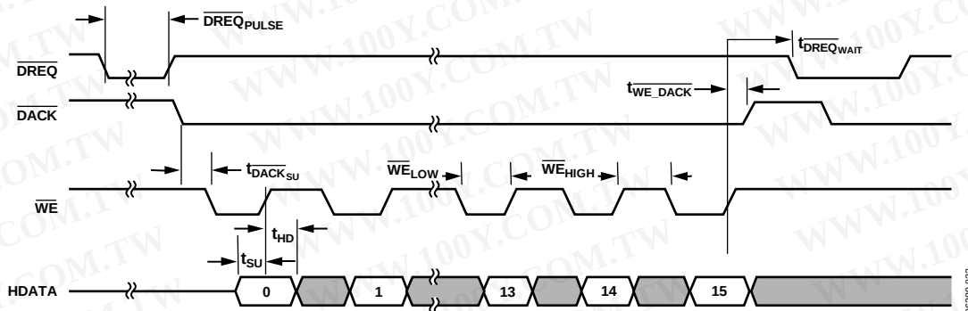
Figure 13. Burst Write Cycle for DREQ/DMA Mode for Assigned DMA Channel (EDMOD0/EDMOD1[14:1] Not Programmed to a Value of 0000)
