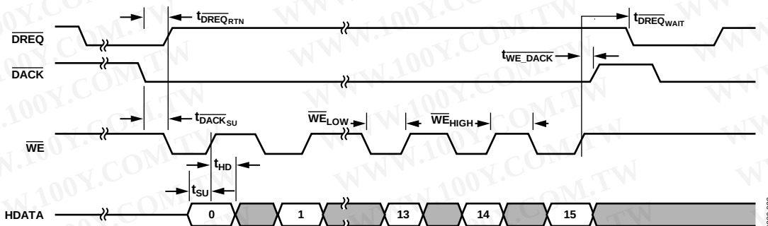
Figure 14. Burst Write Cycle for DREQ/DMA Mode for Assigned DMA Channel (EDMOD0/EDMOD1[14:1] Programmed to a Value of 0000)
