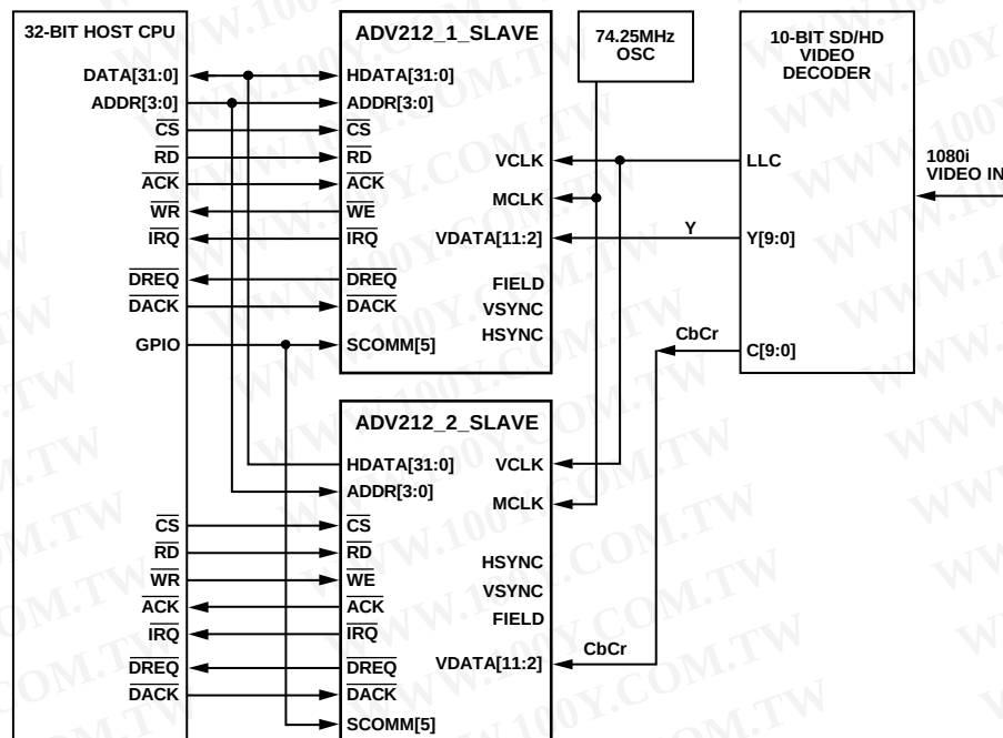
Figure 33. Encode—Multichip Application
