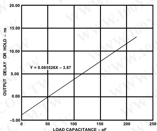
Figure 35. Typical Output Delay or Hold vs. Load Capacitance (at Max Case Temperature)
