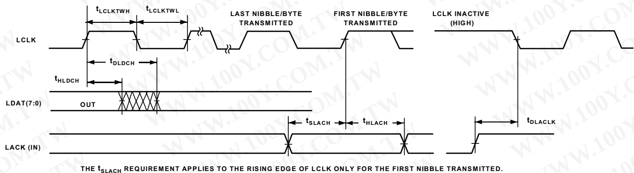
Figure 25. Link Ports—Transmit
