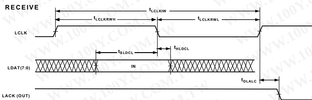
Figure 24. Link Ports—Receive
