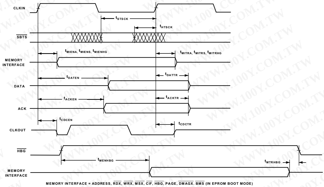
Figure 22. Three-State Timing—Bus Slave, \overline{HBR} , \overline{SBTS}
