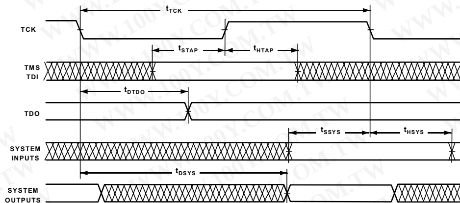
Figure 28. IEEE 1149.1 JTAG Test Access Port
