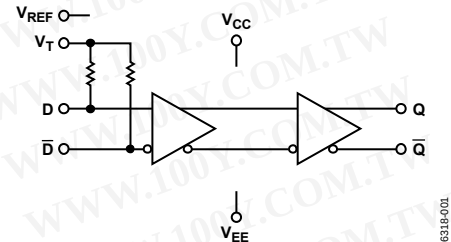
Figure 1. ADCLK905 ECL 1:1 Clock/Data Buffer
