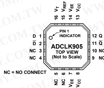
Figure 4. ADCLK905 Pin Configuration
