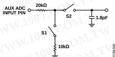
Figure 31. Auxiliary ADC Input Circuit
