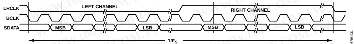
Figure 32. I²S Mode—16 Bits to 24 Bits Per Channel
