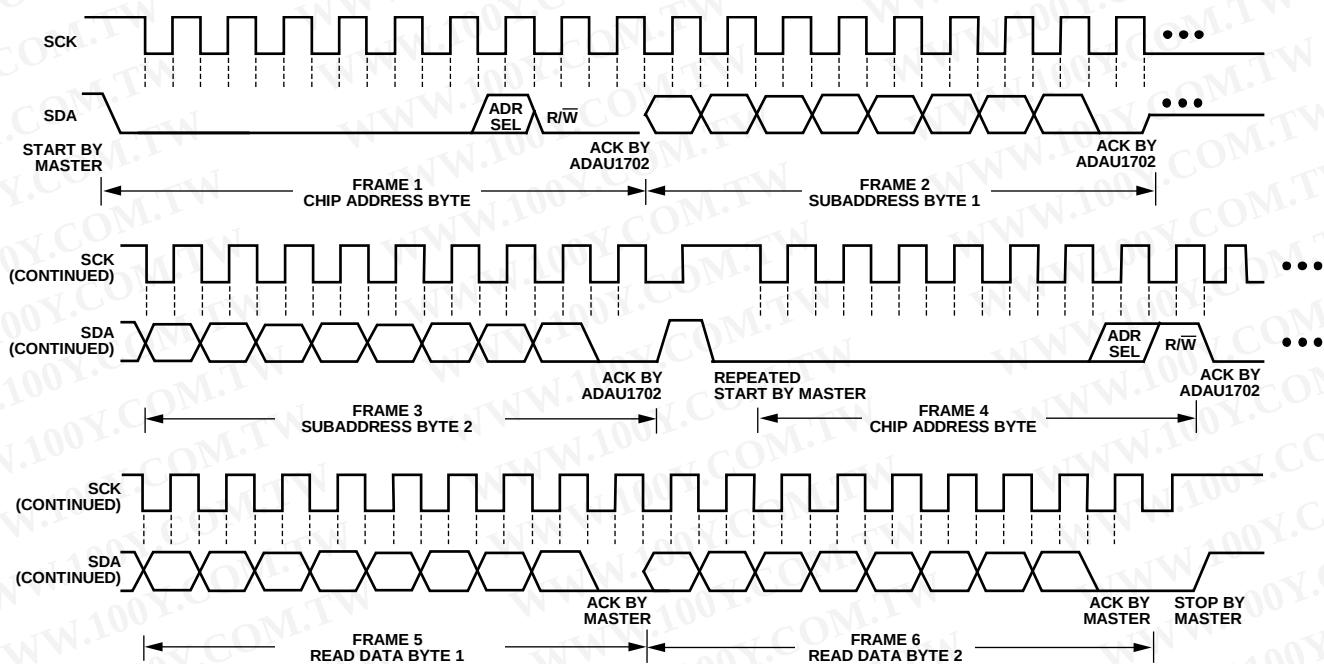
Figure 21. I 2 C Read from ADAU1702 Clocking
