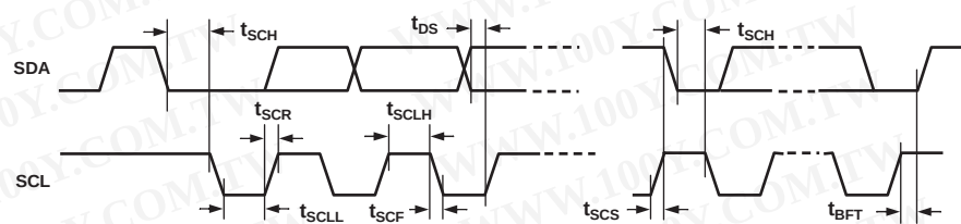
Figure 4. I²C Port Timing
