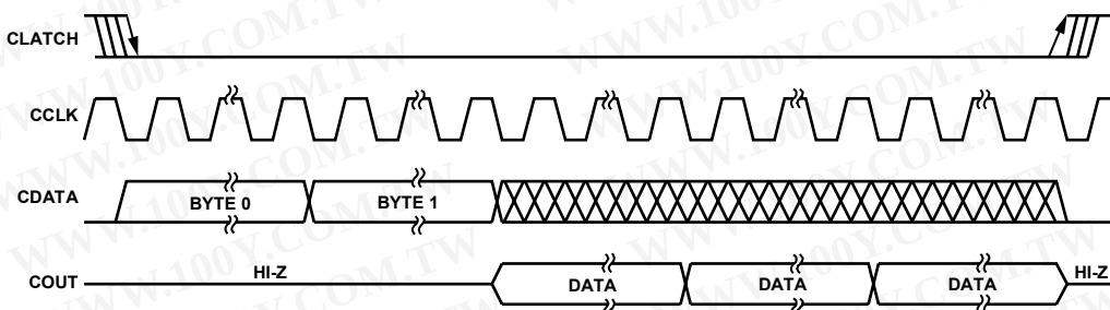
Figure 27. SPI Read from ADAU1701 Clcking (Single-Read Mode)
