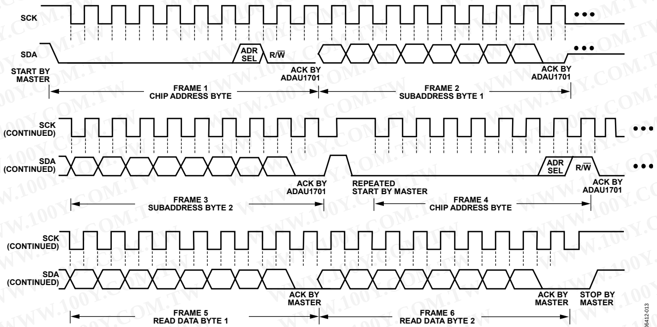
Figure 21. I 2 C Read from ADAU1701 Clocking
