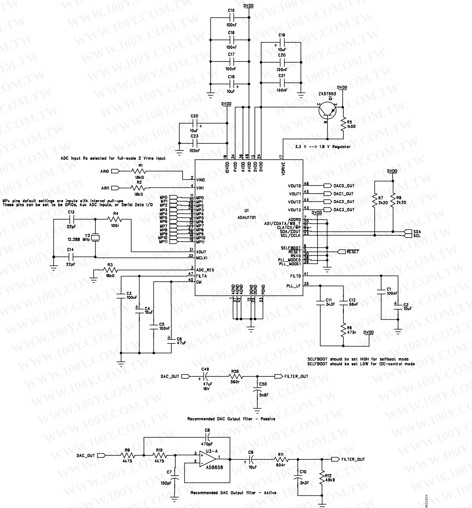
Figure 37. I 2 C Control Schematic
