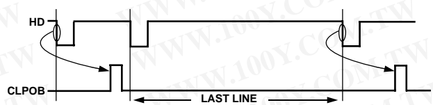
Figure 24. Last HD Longer than Regular HD
