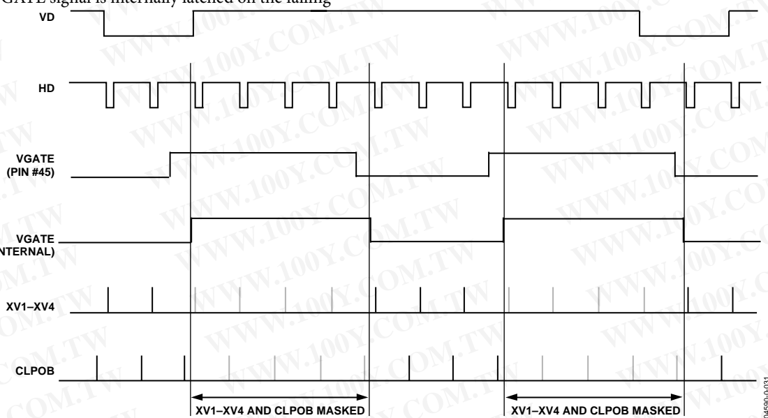
Figure 30. Example of VGATE Input Masking V1 to V4 and CLPOB Outputs with MSHUT/VGATE_EN = 0
