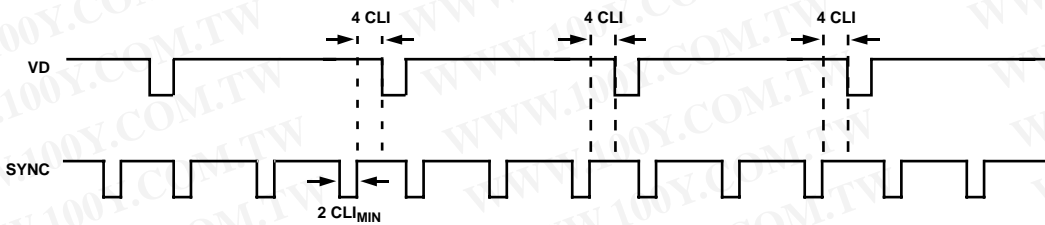
Figure 21. Example of Synchronization with SYNCPOL = 0 and SYNCCNT = 3
