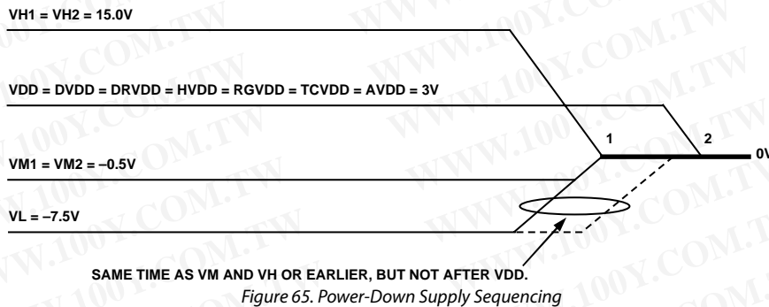
Figure 65. Power-Down Supply Sequencing
