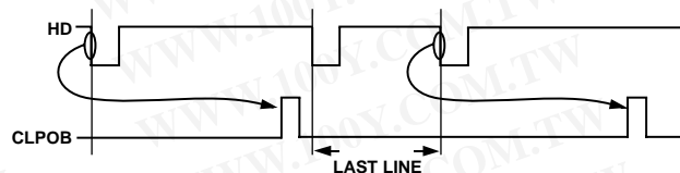
Figure 23. Last HD Shorter than Regular HD
