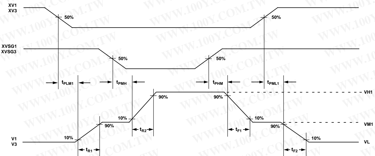
Figure 42. V1 and V3 Transmission Delays and Rise Times
