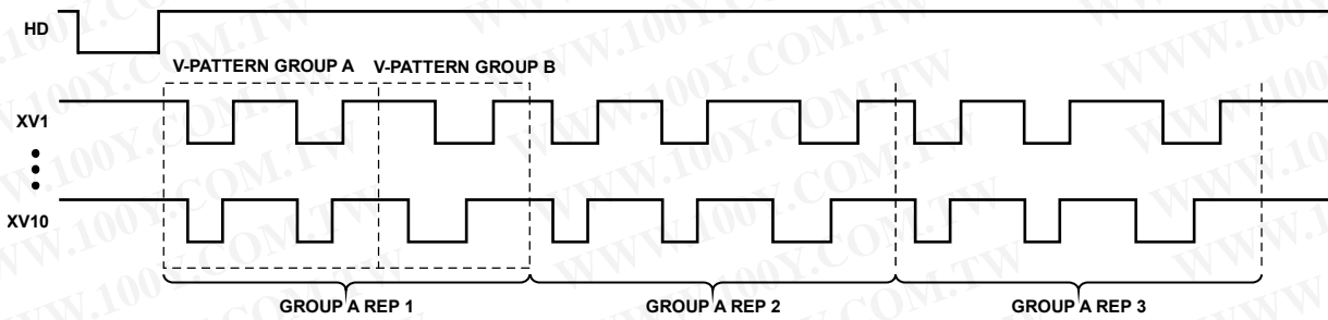
Figure 39. Combining Group A and Group B Patterns with Repetition
