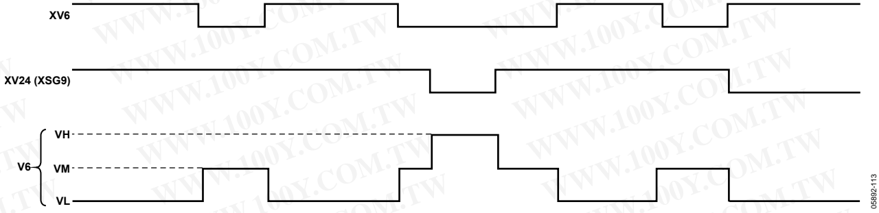
Figure 62. XV6, XV24, and V6 Output Polarities
