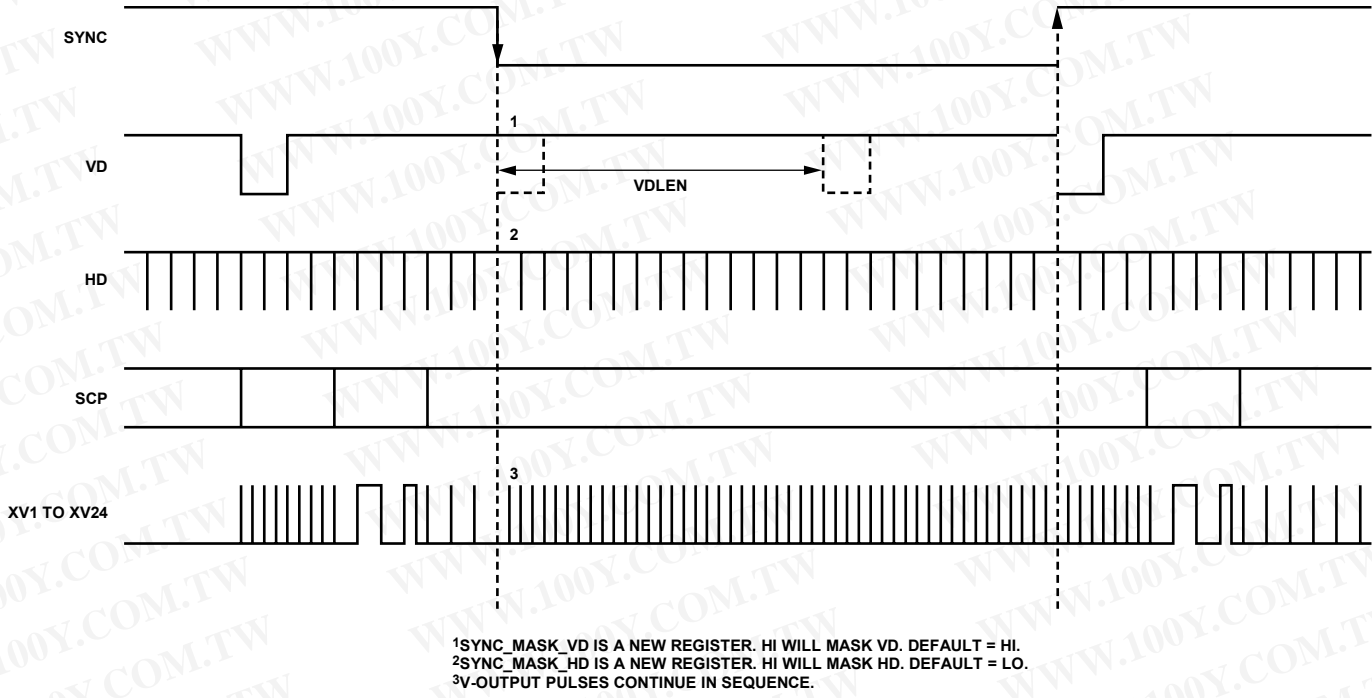
Figure 81. Enhanced SYNC Mode 3
