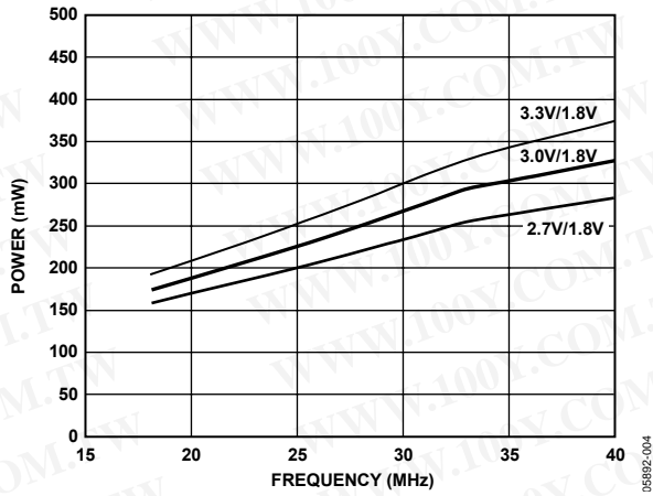
Figure 4. AFETG Power vs. Frequency (V-Driver not Included) (AVDD = TCVD = DVDD = 1.8 V, All Other Supplies at 2.7 V, 3.0 V, or 3.3 V)
