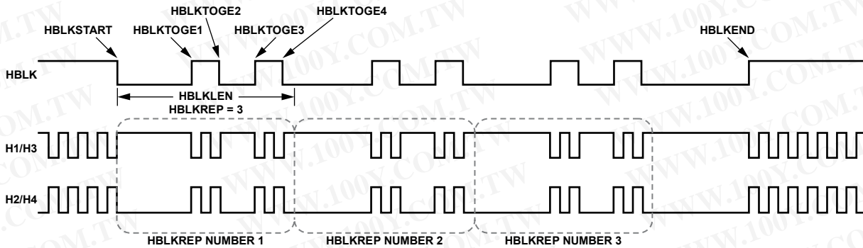
H-BLANK REPEATING PATTERN IS CREATED USING HBLKLEN AND HBLKREP REGISTERS Figure 28. HBLK Repeating Pattern Using HBLKMODE = 1
