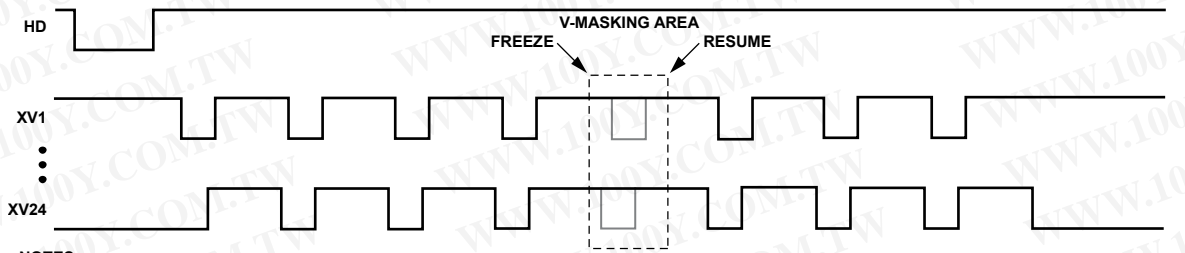
Figure 45. Using FREEZE/RESUME
