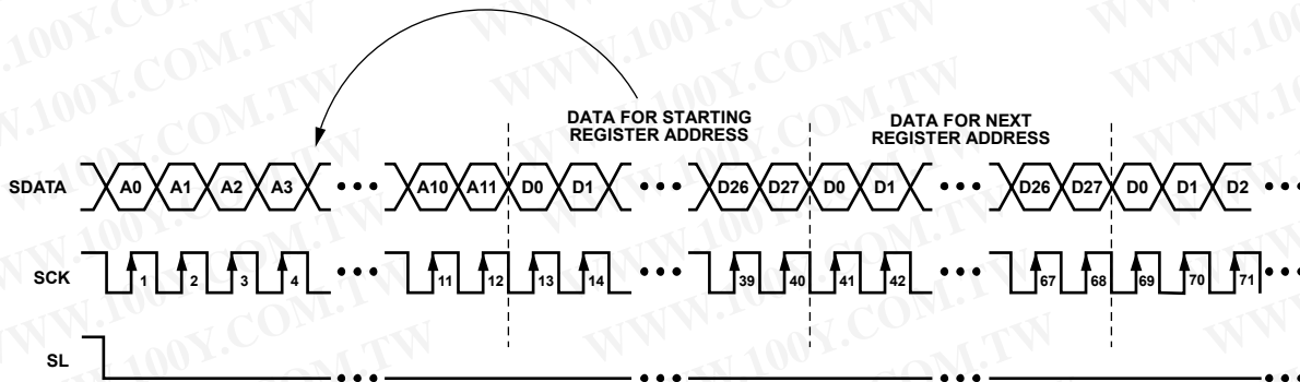
Figure 97. Serial Write Operation
