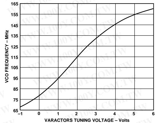
Figure 11. VCO Frequency vs. Voltage
