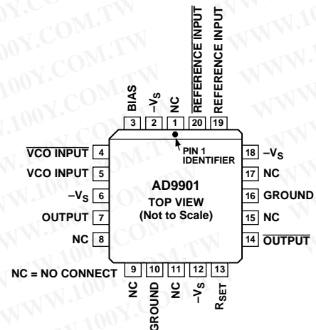
ECL PLCC Pinouts
