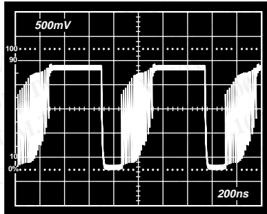
Figure 8. AD9901 Output Waveform ( F_0 \ll F_I )
