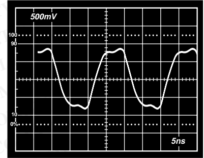
Figure 10. AD9901 Output Waveform ( F_0 = F_I = 50 \text{ MHz} )
