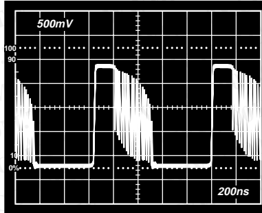
Figure 9. AD9901 Output Waveform ( F_0 \gg F_I )
