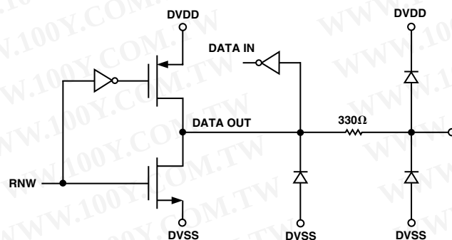
Figure 4. SDATA (Pin 47)
