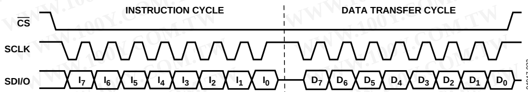
Figure 42. 2-Wire Serial Port Read Timing—Clock Stall High
