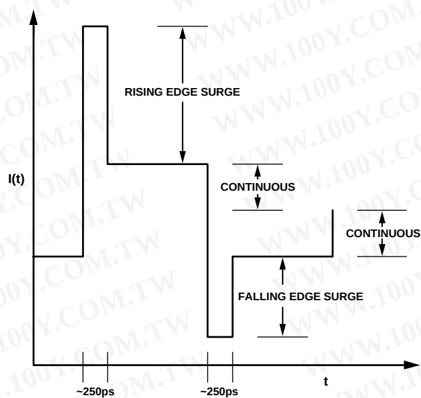
Figure 37. Rising Edge and Falling Edge Surge Current Out of the CML Clock Driver, as Opposed to the Steady State Continuous Current
