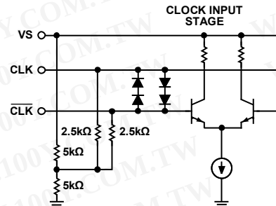
Figure 36. CLK Equivalent Input Circuit
