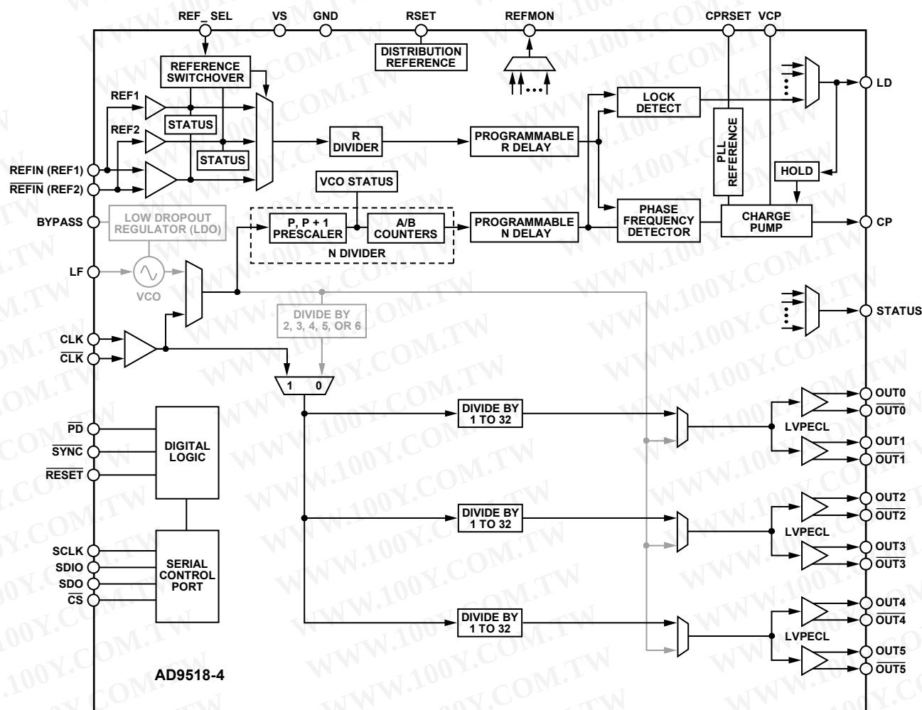
Figure 29. Clock Distribution or External VCO &lt; 1600 MHz
