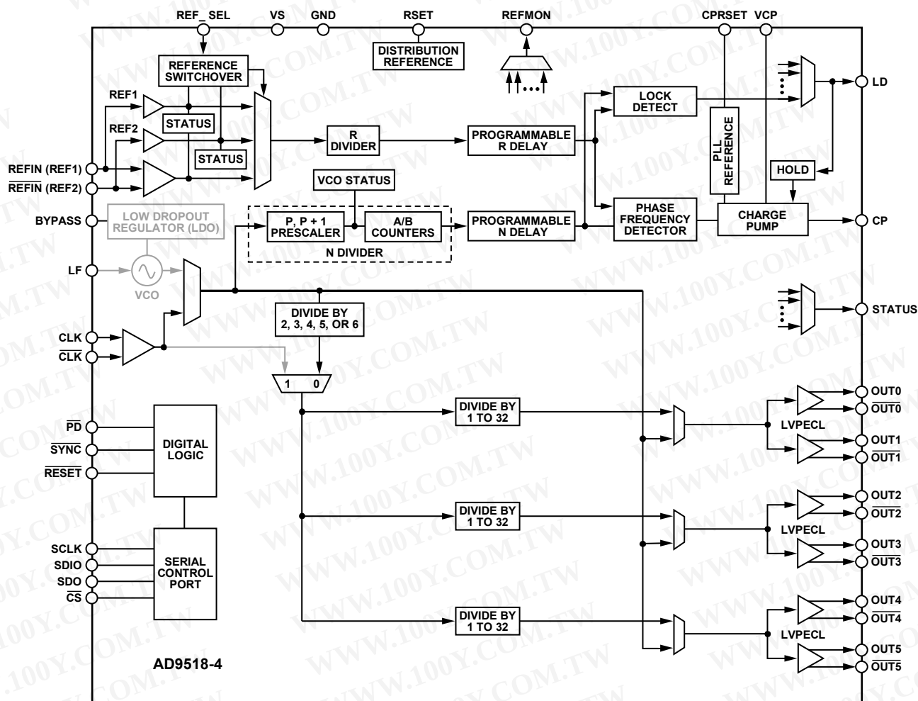
Figure 27. High Frequency Clock Distribution or External VCO &gt; 1600 MHz
