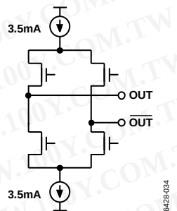
Figure 59. LVDS Output Simplified Equivalent Circuit with 3.5 mA Typical Current Source
