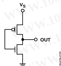
Figure 60. CMOS Equivalent Output Circuit
