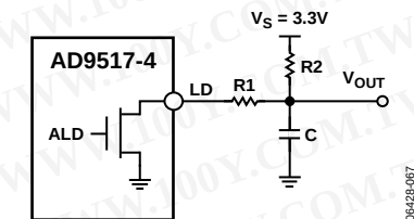
Figure 49. Example of Analog Lock Detect Filter Using an N-Channel Open-Drain Driver
