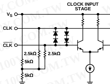
Figure 51. CLK Equivalent Input Circuit
