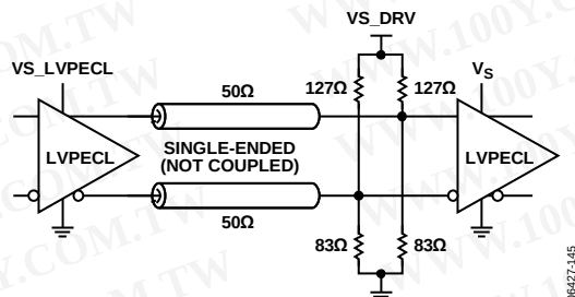
Figure 70. DC-Coupled 3.3 V LVPECL Far-End Thevenin Termination
