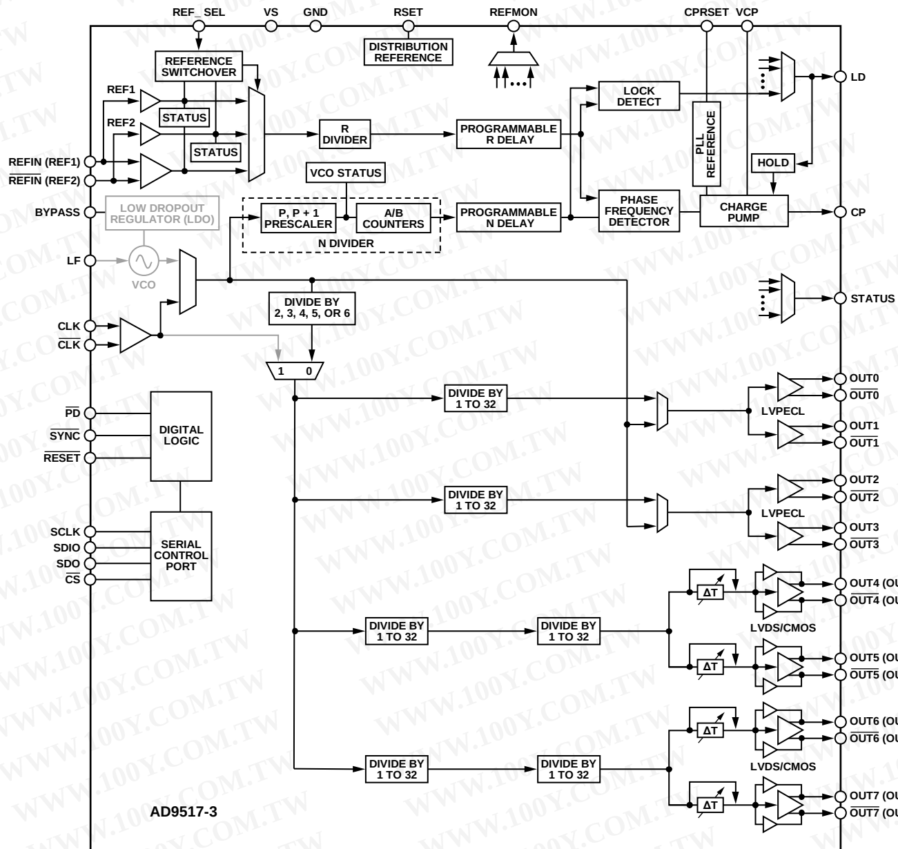
Figure 42. High Frequency Clock Distribution or External VCO > 1600 MHz
