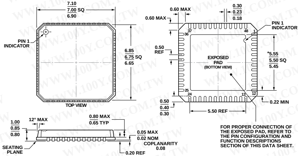
Figure 76. 48-Lead Lead Frame Chip Scale Package [LFCSP_VQ] 7 mm x 7 mm Body, Very Thin Quad CP-48-8 Dimensions shown in millimeters
