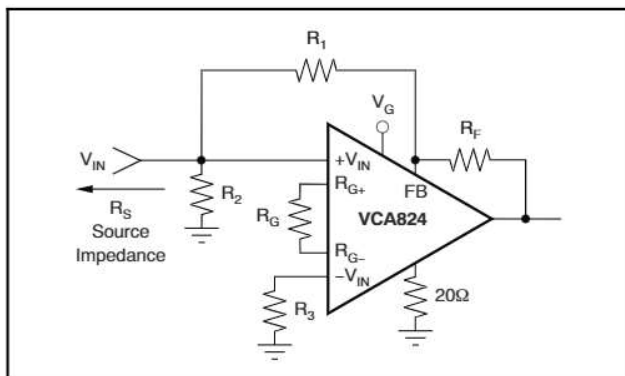
Figure 76. Four-Quadrant Multiplier Circuit
