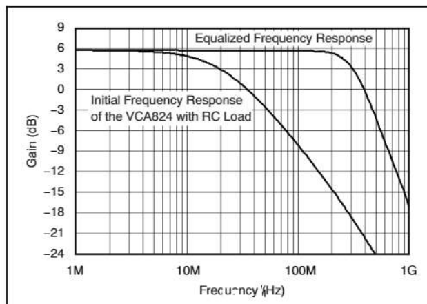
Figure 81. Differential Equalization of an RC Load
