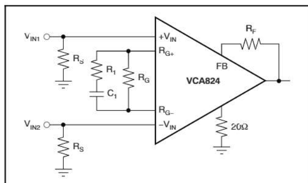
Figure 80. Differential Equalizer
