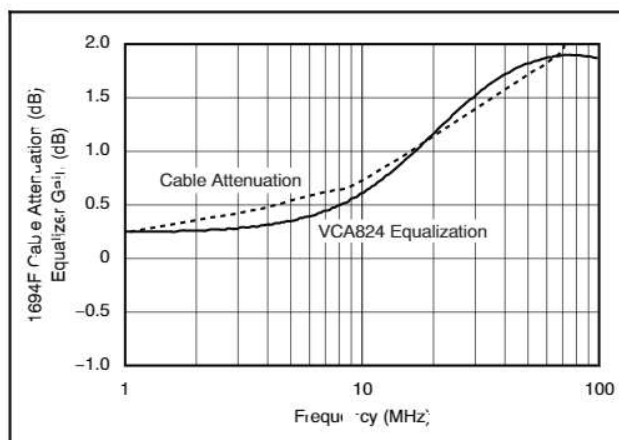
Figure 82. Cable Attenuation versus Equalizer Gain
