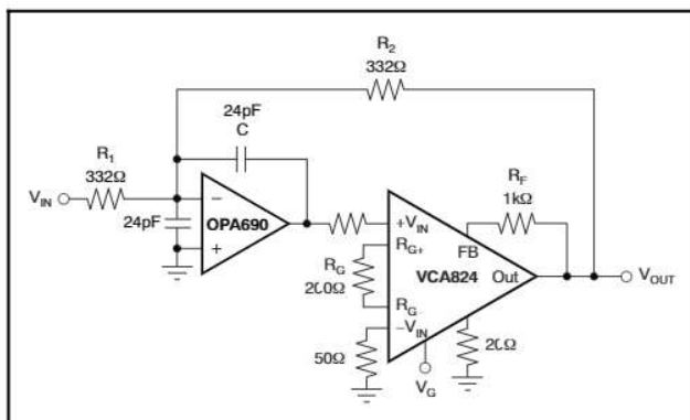
Figure 84. Voltage-Control Low-Pass Filter
