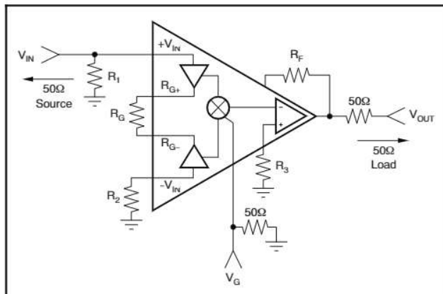
Figure 85. Test Circuit
