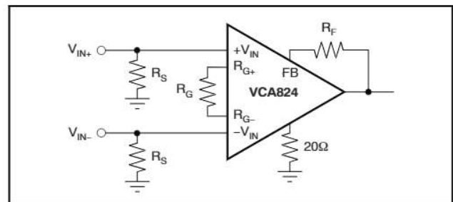
Figure 78. Difference Amplifier
