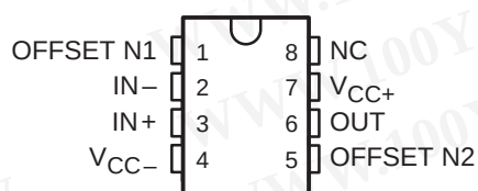
\mu A741M . . . U PACKAGE
