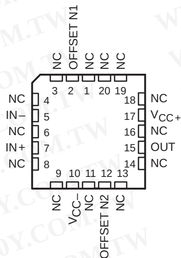
\mu A741M . . . FK PACKAGE
